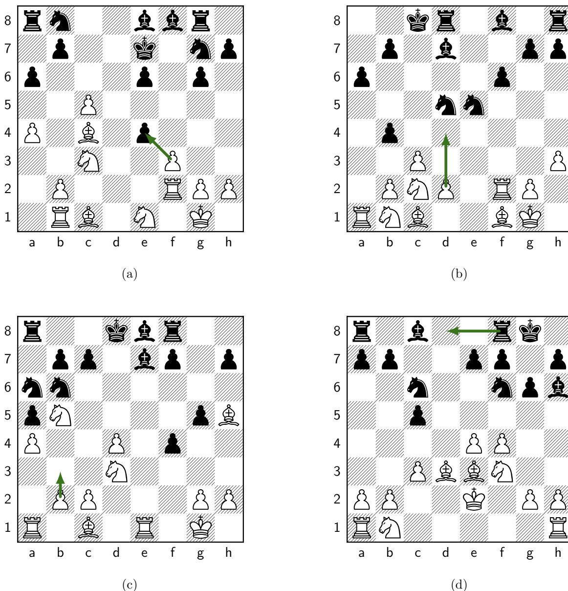
Figure 12: Move 18, White: fxe4 . (a) Our position; Melanie plays fxe4 ( f3e4 ). Panels (b)–(d) are the retrieved master positions whose correspondence most drove this move (highest QAP objective among those that transfer to it). (b) Retrieved from ccr1_top_p0000#2781 (ply 34) [structural distance d=100 , QAP obj=88]: the master played d4 ; under \mu our Rf2 plays the role of that game’s Pd2 (a cross-type correspondence); cross-type roles: our Bc1 as their Ra1 , our pa6 as their Bc1 ; transferred move f2e2 . (c) Retrieved from ccr1_top_p0002#1064 (ply 32) [structural distance d=105 , QAP obj=67]: the master played b3 ; under \mu our Pc5 plays the role of that game’s Pb2 ; cross-type roles: our Pa4 as their Bc1 , our Bc4 as their Re1 ; transferred move c5c6 . (d) Retrieved from ccr1_top_p0002#3362 (ply 19) [structural distance d=89 , QAP obj=47]: the master played Rd8 ; under \mu our Rf2 plays the role of that game’s Rf1 ; cross-type roles: our Ne1 as their Ra8 , our Pg2 as their Bc8 ; transferred move f2c2 . Synthesis: no retrieved analog transferred to fxe4 – the search selector chose it on value (material / mate); panels (b)–(d) show the strongest nearby analogies.
