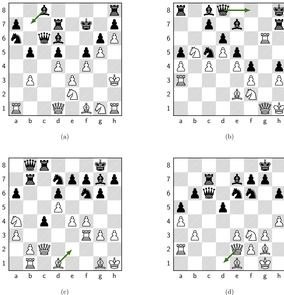
Figure 33: Move 39, Black: Bb7 . (a) Our position; Melanie plays Bb7 (c8b7). Panels (b)–(d) are the retrieved master positions whose correspondence most drove this move (highest QAP objective among those that transfer to it). (b) Retrieved from ccr1_top_p0000#947 (ply 61) [structural distance d=140 , QAP obj=70]: the master played Qf8; under \mu our Bc1 plays the role of that game’s Qd1 (a cross-type correspondence); cross-type roles: our ng1 as their Ra8, our Pd5 as their Bc8; transferred move c8b7 ( endorses this move ). (c) Retrieved from ccr1_top_p0003#53 (ply 86) [structural distance d=132 , QAP obj=45]: the master played Be2; under \mu our Bc1 plays the role of that game’s Bd1; cross-type roles: our qd1 as their Rb1, our Rh8 as their Bg1; transferred move c8b7 ( endorses this move ). (d) Retrieved from ccr1_top_p0000#3209 (ply 66) [structural distance d=141 , QAP obj=34]: the master played Qd1; under \mu our Bc1 plays the role of that game’s Qe2 (a cross-type correspondence); cross-type roles: our Qc6 as their Ra2, our Pa7 as their Bg2; transferred move c8b7 ( endorses this move ). Synthesis: 9 retrieved analogs transferred to Bb7 (summed QAP objective 262, the strongest correspondence among the candidate moves); Melanie committed it via the search selector.
