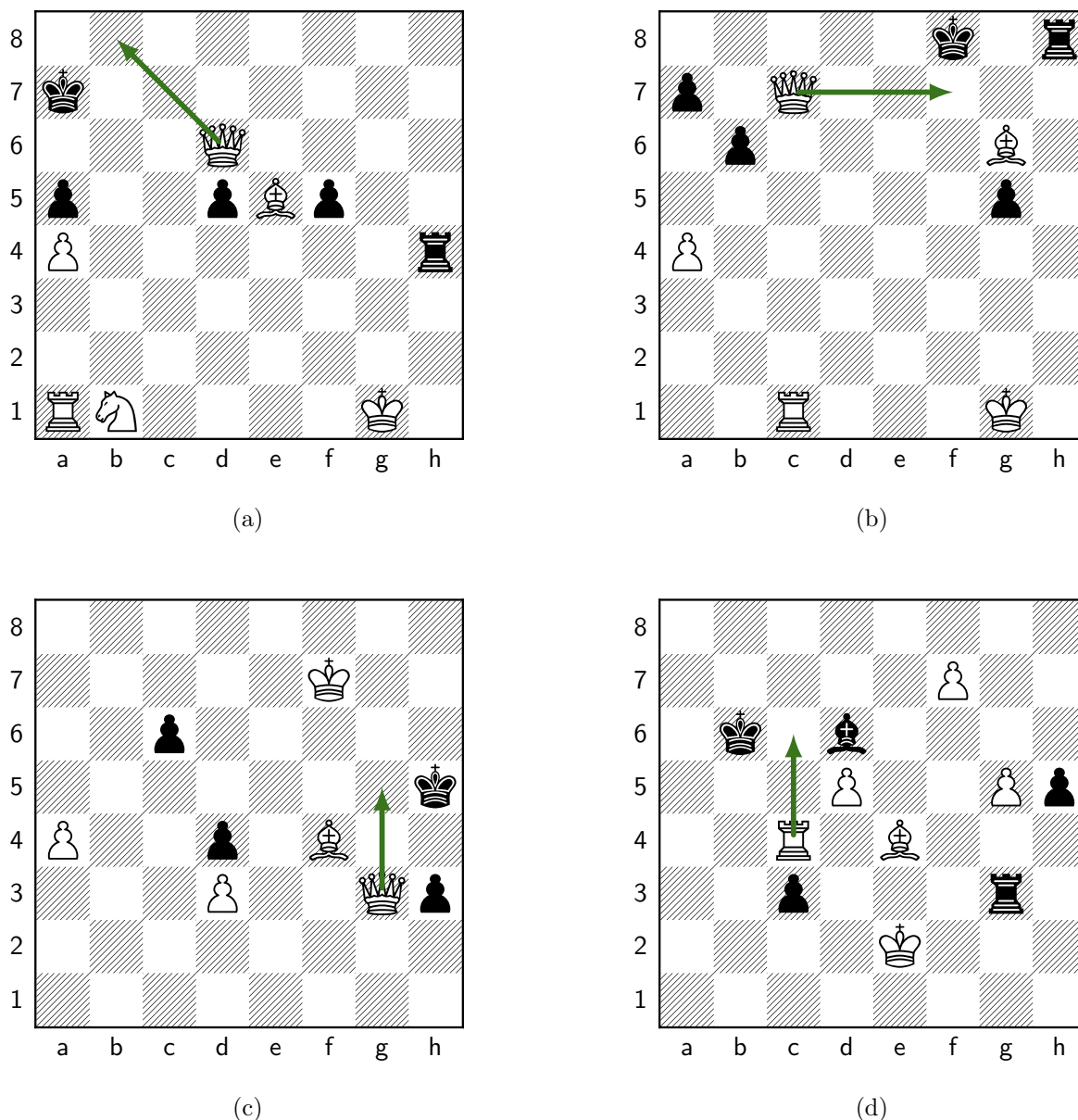
Figure 56: Move 62, White: Qb8+. (a) Our position; Melanie plays Qb8+ (d6b8). Panels (b)–(d) are the retrieved master positions whose correspondence most drove this move (highest QAP objective among those that transfer to it). (b) Retrieved from lichess_elite_2024-09_p0028#219 (ply 106) [structural distance d=30 , QAP obj=25]: the master played Qf7#; under \mu our Qd6 plays the role of that game’s Qc7; cross-type roles: our Be5 as their Rc1, our Nb1 as their Pa4; transferred move d6a6. (c) Retrieved from lichess_elite_2024-09_p0028#1132 (ply 122) [structural distance d=32 , QAP obj=23]: the master played Qg5#; under \mu our Qd6 plays the role of that game’s Qg3; cross-type roles: our Nb1 as their Pd3, our rh4 as their pd4; transferred move d6a6. (d) Retrieved from lichess_elite_2024-09_p0030#823 (ply 126) [structural distance d=36 , QAP obj=22]: the master played Rc6+; under \mu our Qd6 plays the role of that game’s Rc4 (a cross-type correspondence); cross-type roles: our Ra1 as their Pd5, our Nb1 as their ph5; transferred move d6a6. Synthesis: no retrieved analog transferred to Qb8+ – the search selector chose it on value (material / mate); panels (b)–(d) show the strongest nearby analogies.
