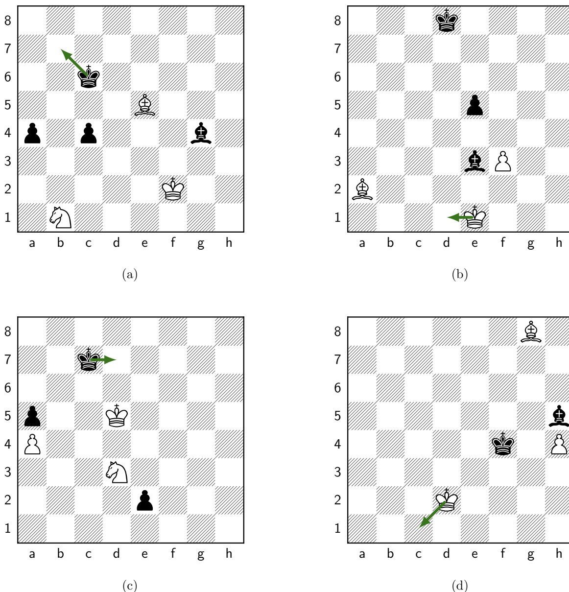
Figure 91: Move 97, Black: Kb7. (a) Our position; Melanie plays Kb7 ( c6b7 ). Panels (b)–(d) are the retrieved master positions whose correspondence most drove this move (highest QAP objective among those that transfer to it). (b) Retrieved from ccr1_top_p0001#1495 (ply 186) [structural distance d=6 , QAP obj=1]: the master played Kd1; under \mu our Kc3 plays the role of that game’s Ke1 ; cross-type roles: our Pa4 as their Ba2 , our nb1 as their pe5 ; transferred move c6b7 (endorses this move) . (c) Retrieved from ccr1_top_p0000#831 (ply 179) [structural distance d=5 , QAP obj=1]: the master played Kd7; under \mu our Kc3 plays the role of that game’s Kc2 ; cross-type roles: our be5 as their pa4 ; transferred move c6b7 (endorses this move) . (d) Retrieved from ccr1_top_p0001#2493 (ply 202) [structural distance d=7 , QAP obj=1]: the master played Kc1; under \mu our Kc3 plays the role of that game’s Kd2 ; cross-type roles: our Bg4 as their Ph4 , our Pc4 as their Bg8 ; transferred move c6b7 (endorses this move) . Synthesis: 18 retrieved analogs transferred to Kb7 (summed QAP objective 15, the strongest correspondence among the candidate moves); Melanie committed it via the search selector.
