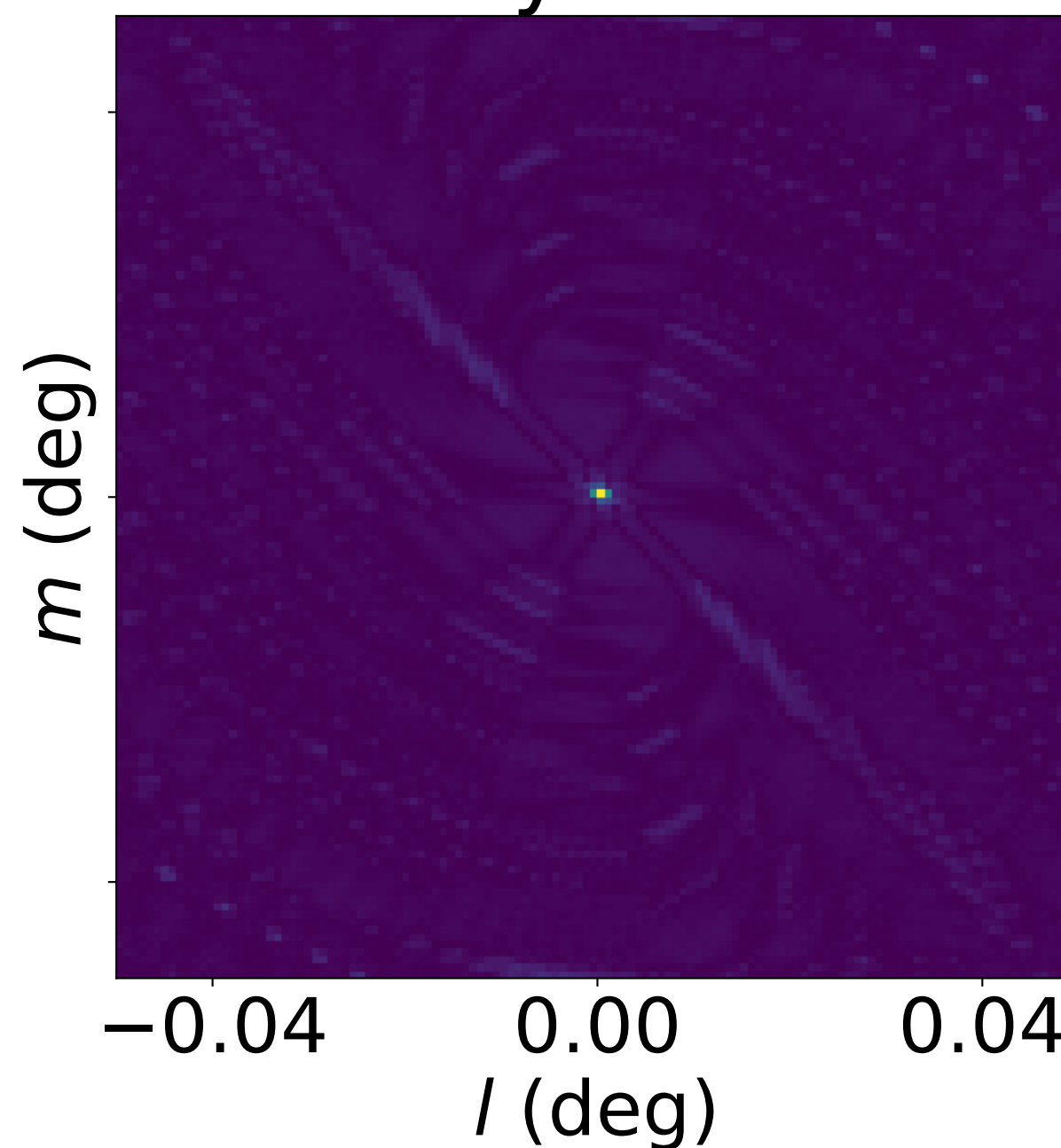
Dirty beam
