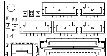
TOP VIEW — 34.25 × 18.50 MM
