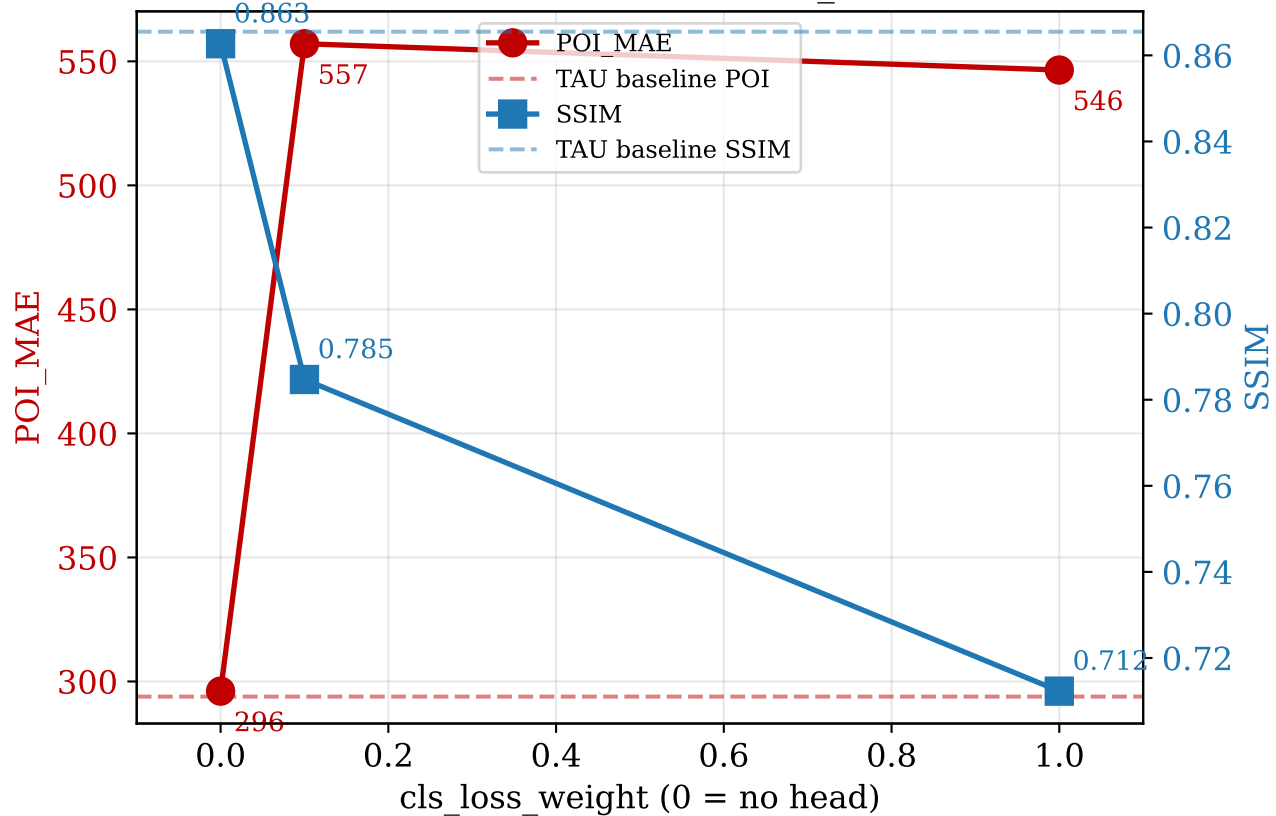
TAU: lowering cls_weight partially recovers SSIM but does NOT restore POI_MAE
