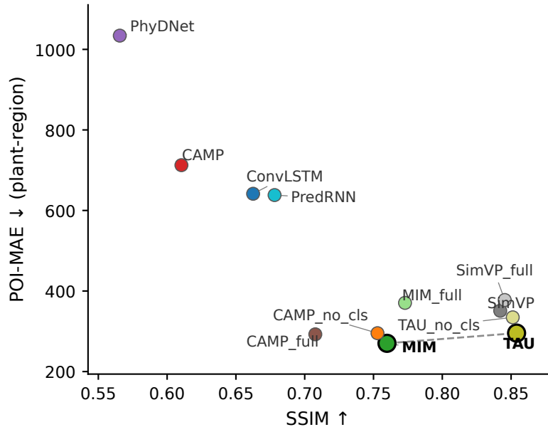
(b) Plant-level: SSIM vs POI-MAE
