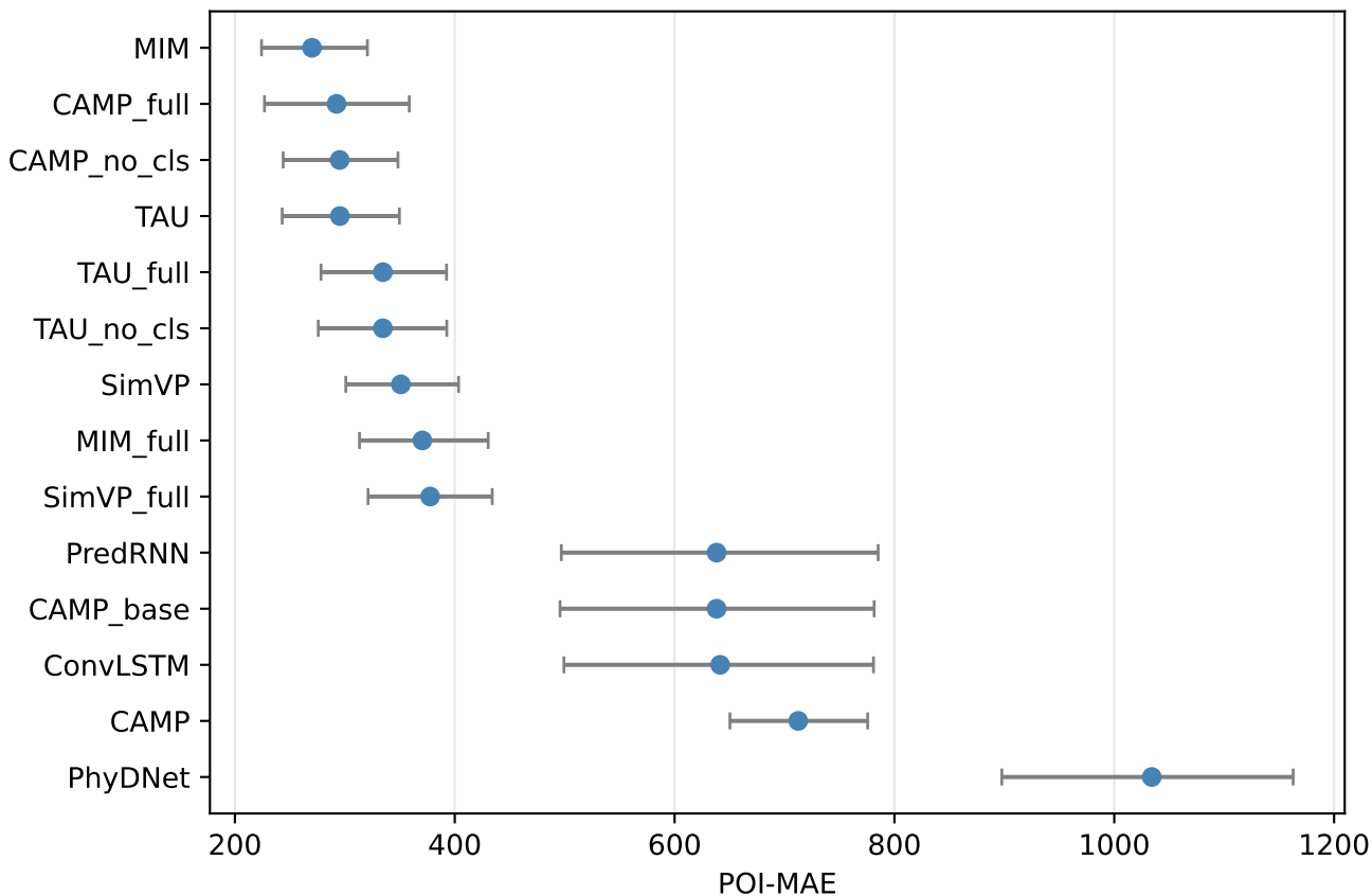
POI-MAE on Komatsuna (95% confidence intervals)
