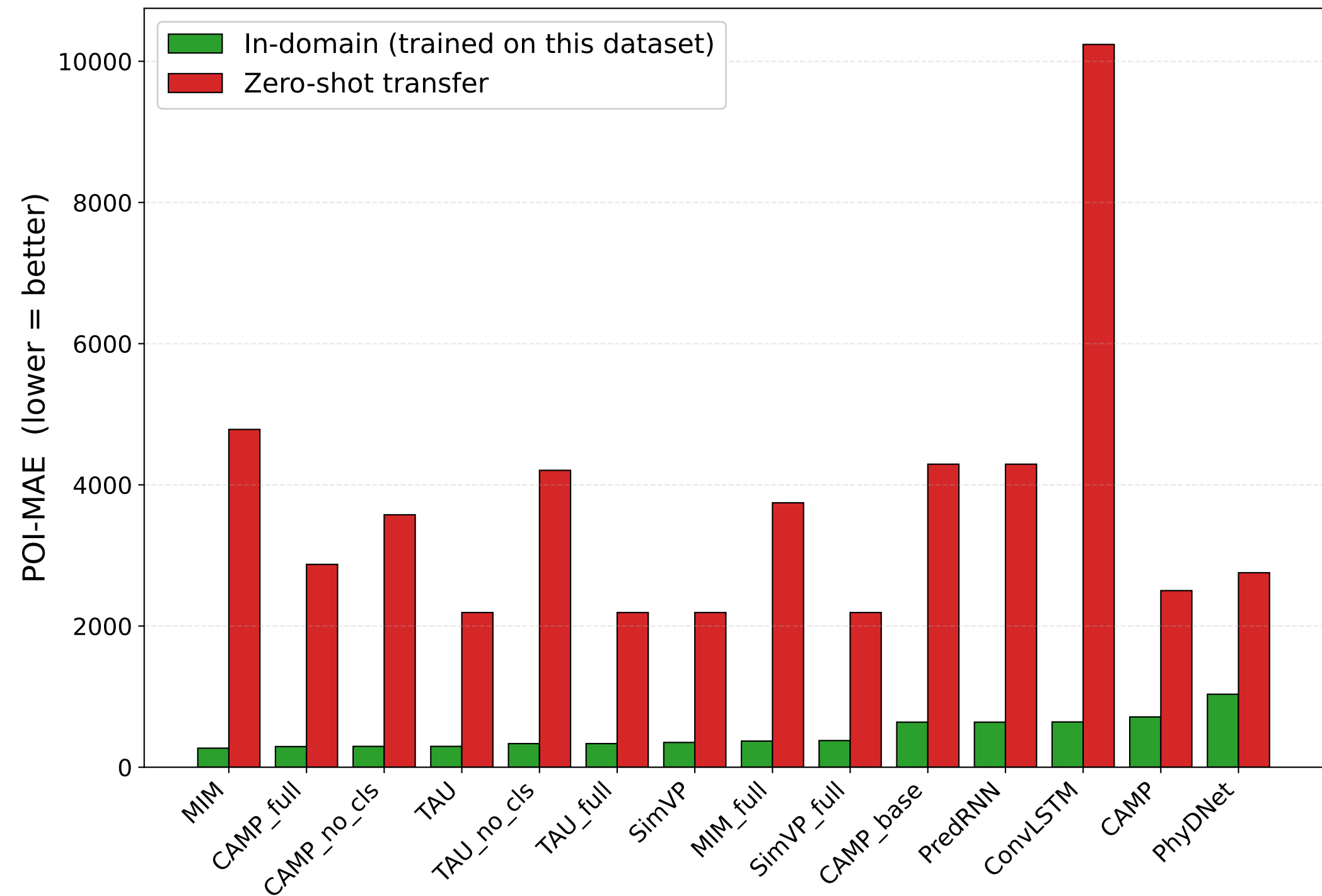
Arabidopsis → Komatsuna transfer (train on Arabidopsis, test on Komatsuna test split, 14 methods)
