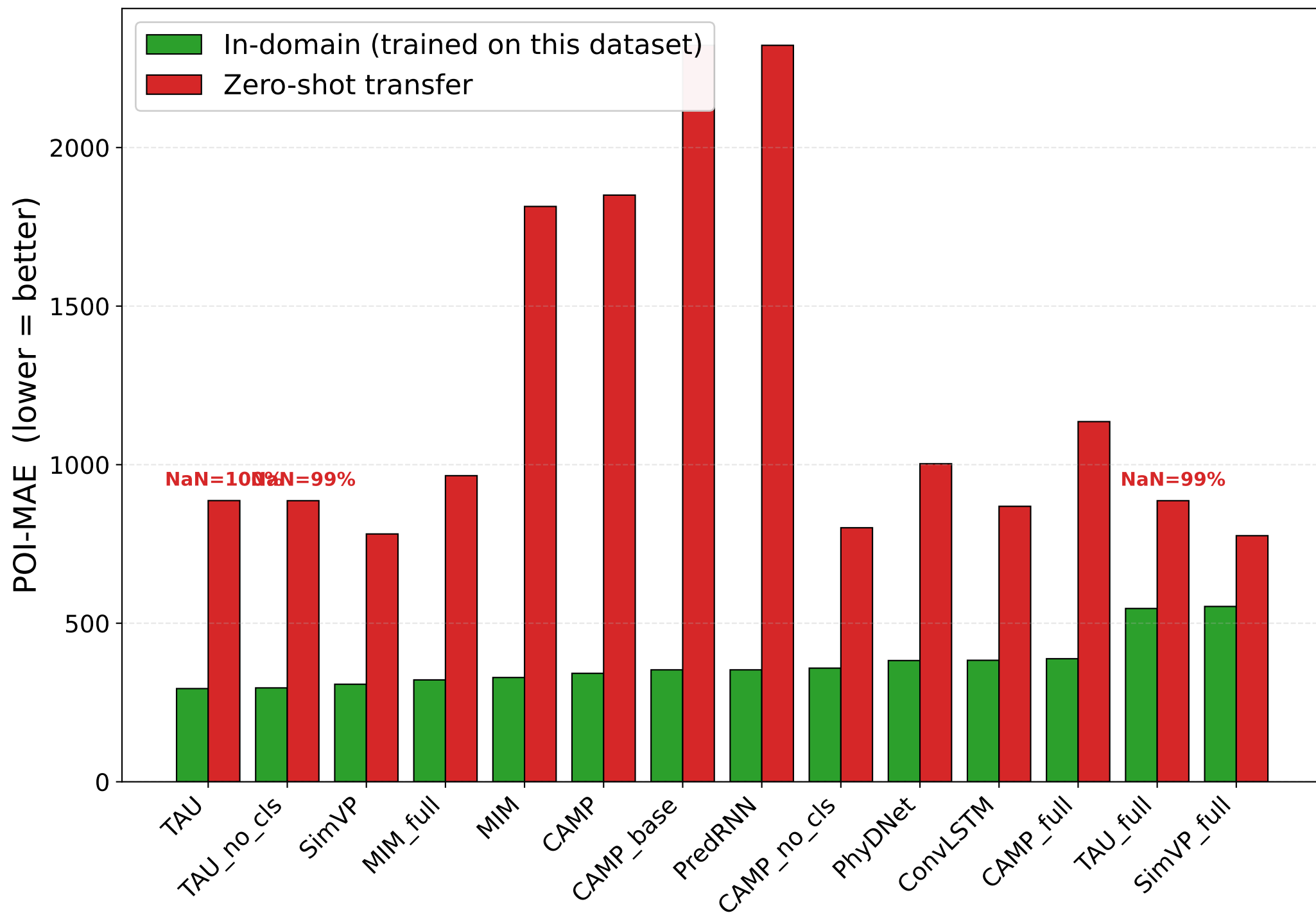
Komatsuna → Arabidopsis transfer (train on Komatsuna, test on Arabidopsis test split, 14 methods)
