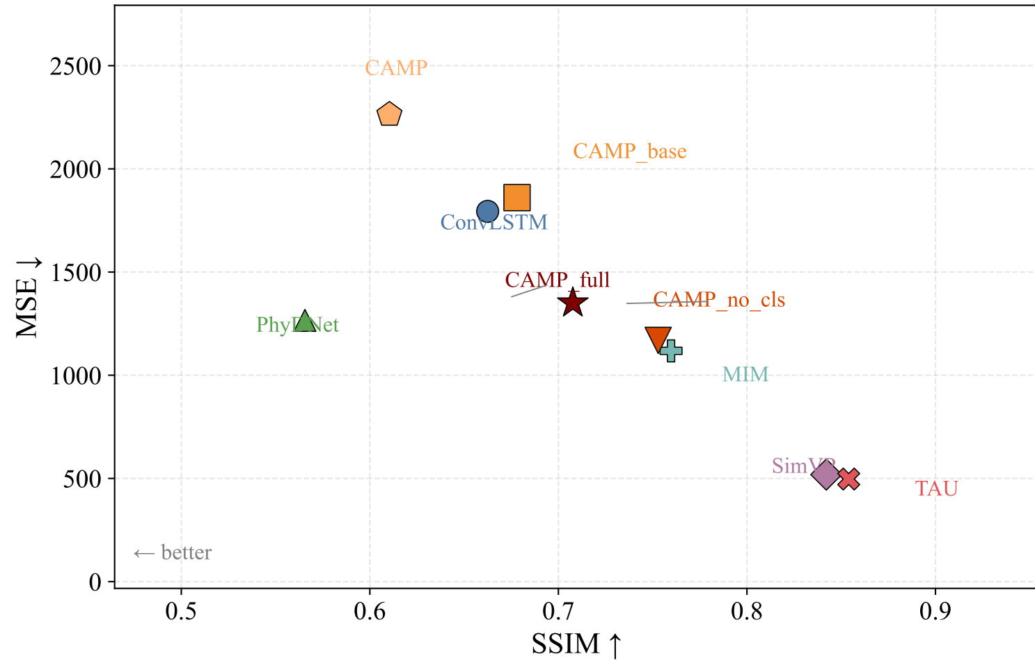
SSIM vs MSE
