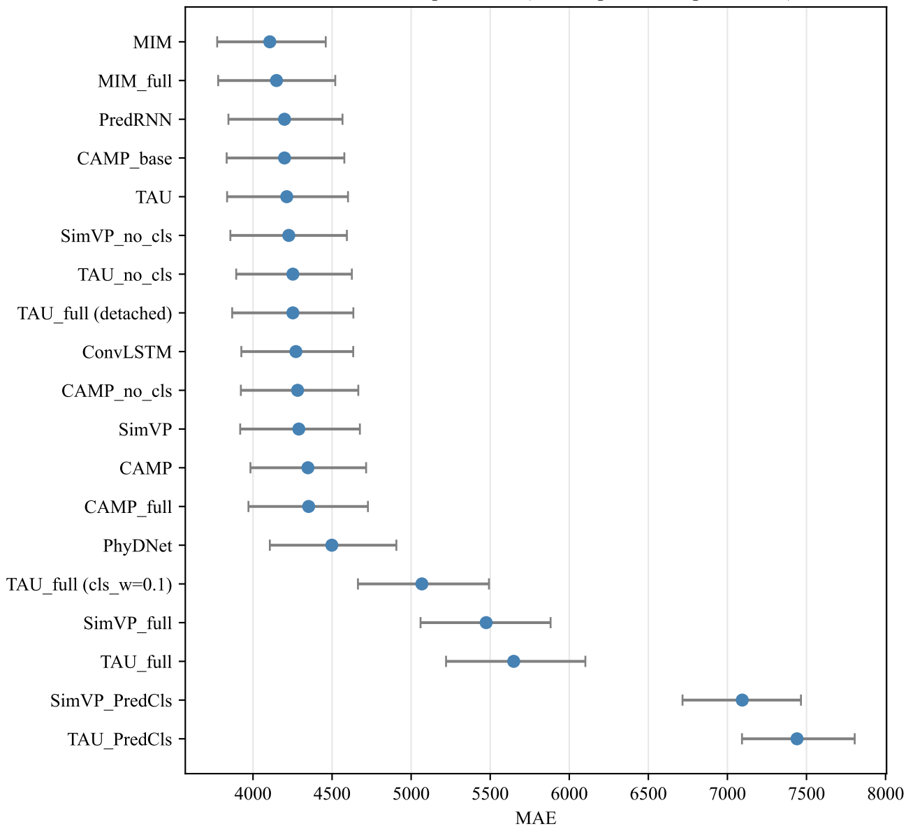
MAE — bootstrap 95% CI (arabidopsis, 150 ep, B=5000)
