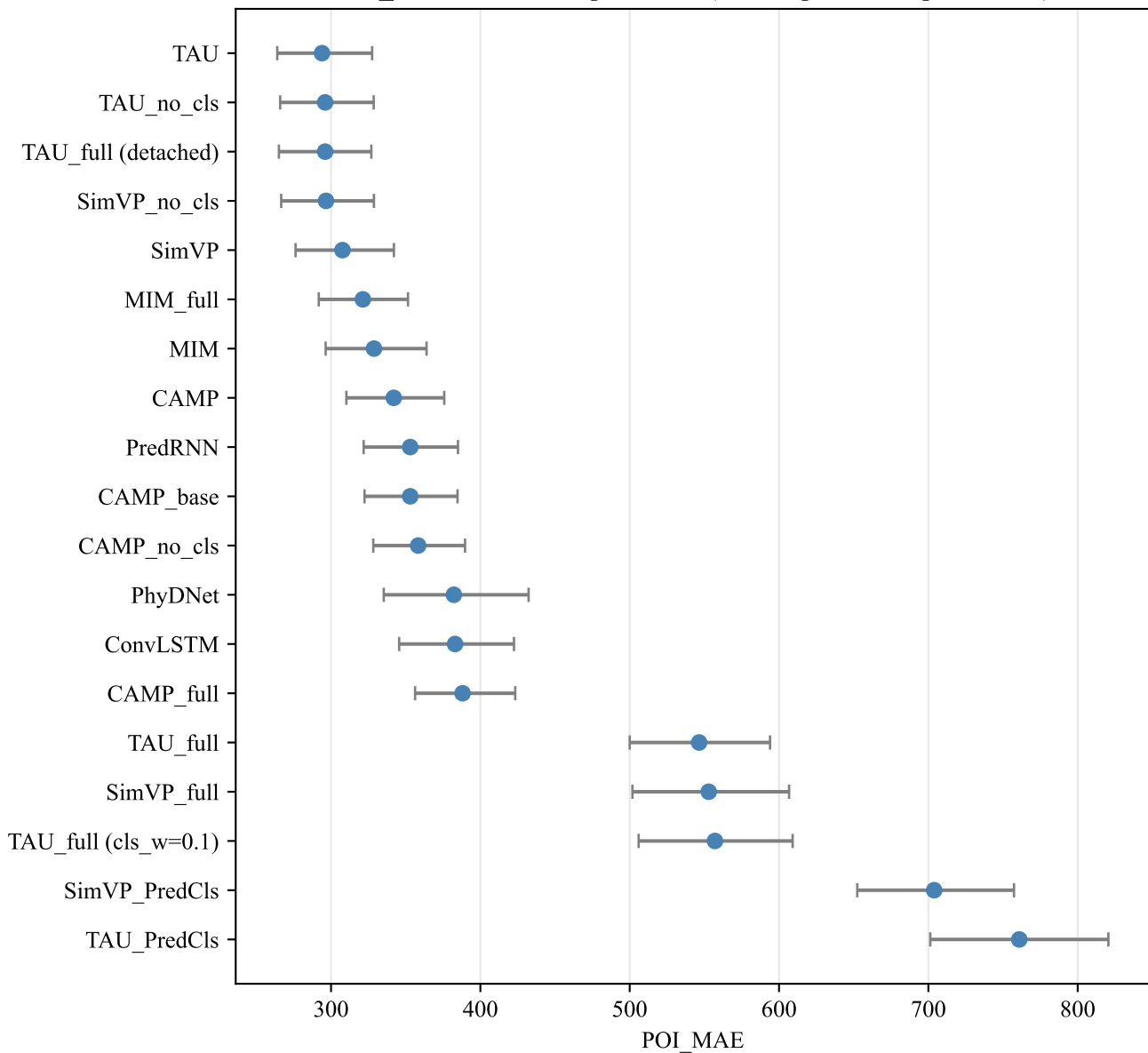
POI_MAE — bootstrap 95% CI (arabidopsis, 150 ep, B=5000)
