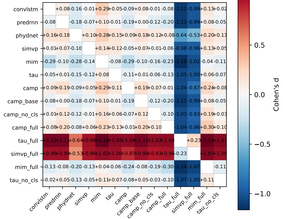
Cohen's d (row vs column) (metric = MAE)
