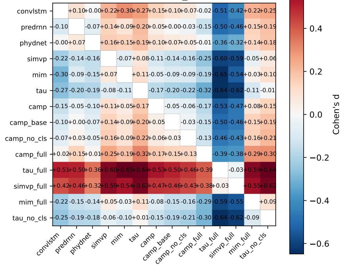
Cohen's d (row vs column) (metric = POI_MAE)
