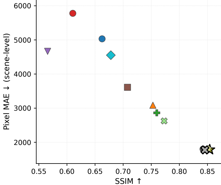
(a) Scene-level: SSIM vs Pixel MAE
