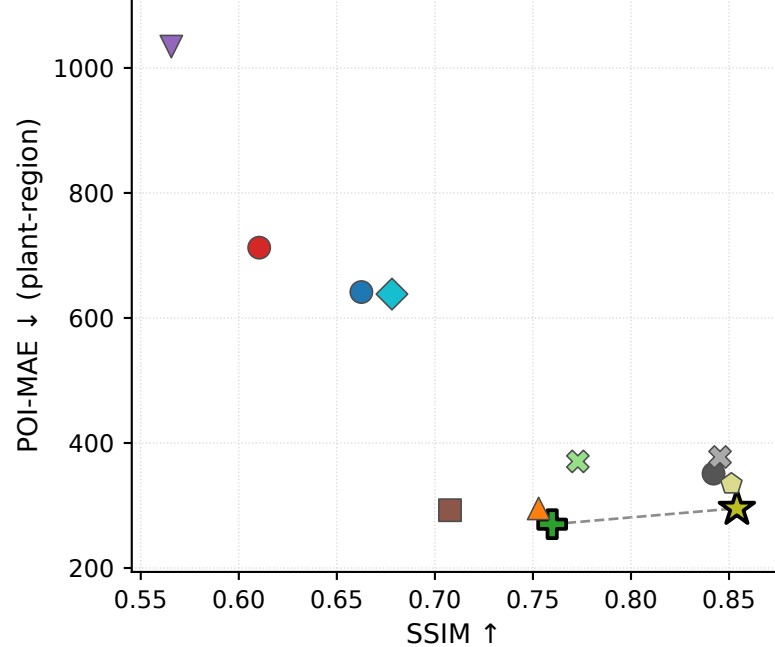
(b) Plant-level: SSIM vs POI-MAE
