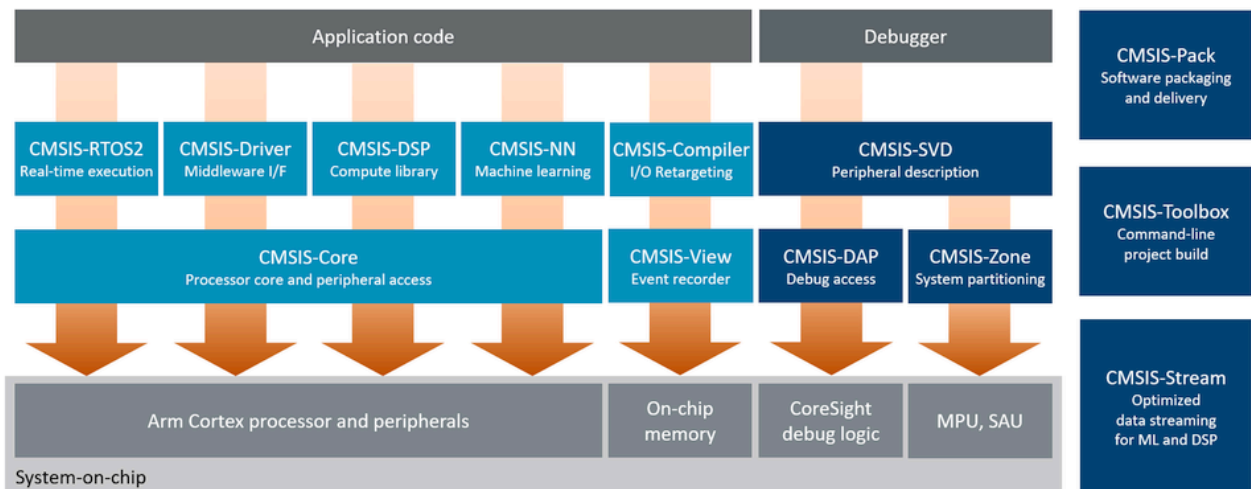
Figure 4-1: CMSIS structure
