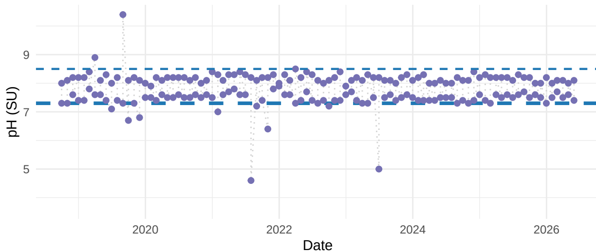
pH over time – External Outfall 002
