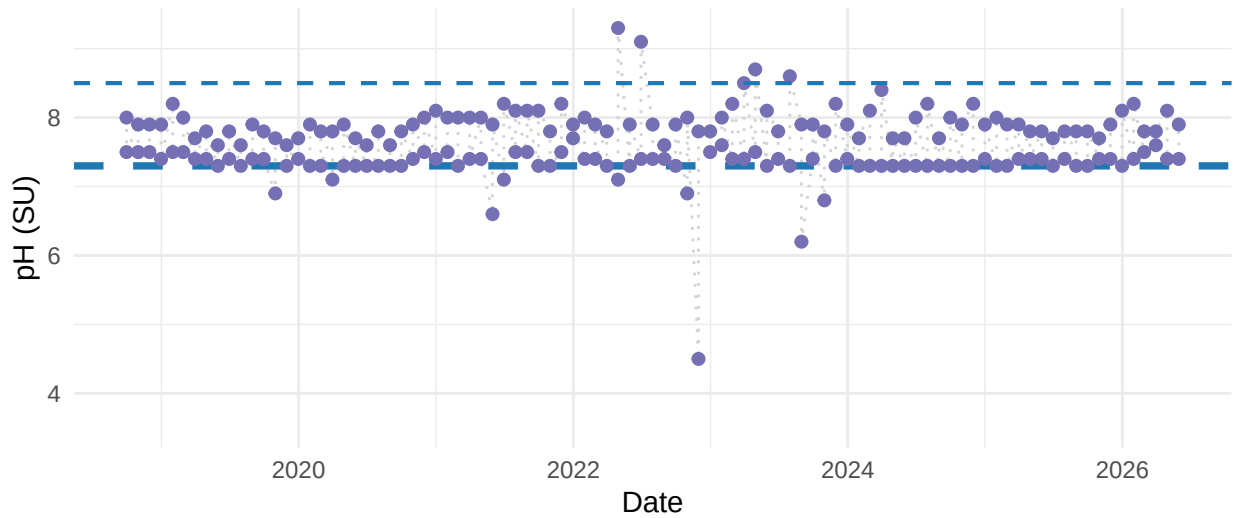
pH over time – External Outfall 003
