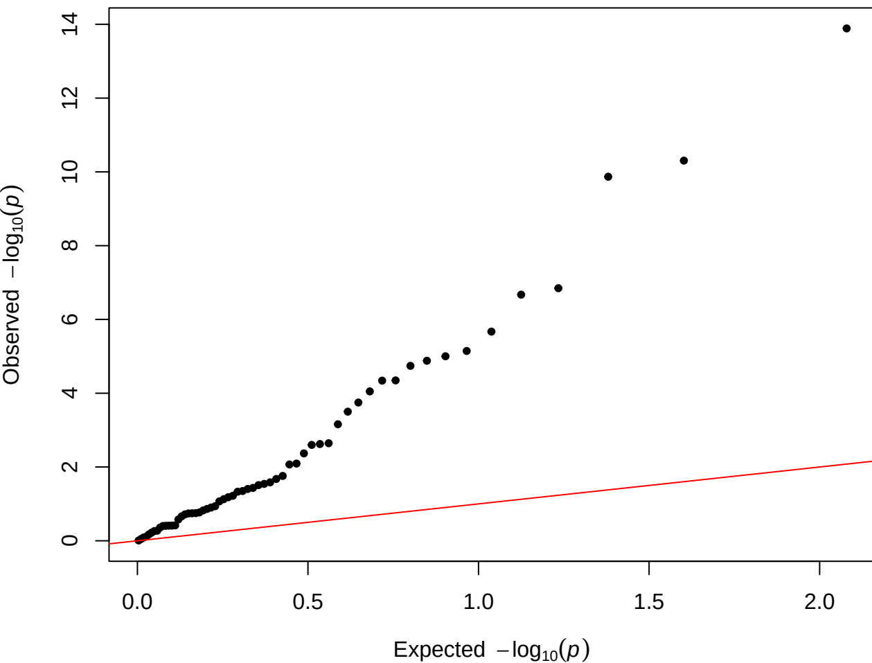
QQ Plot – all, FU=1, full
