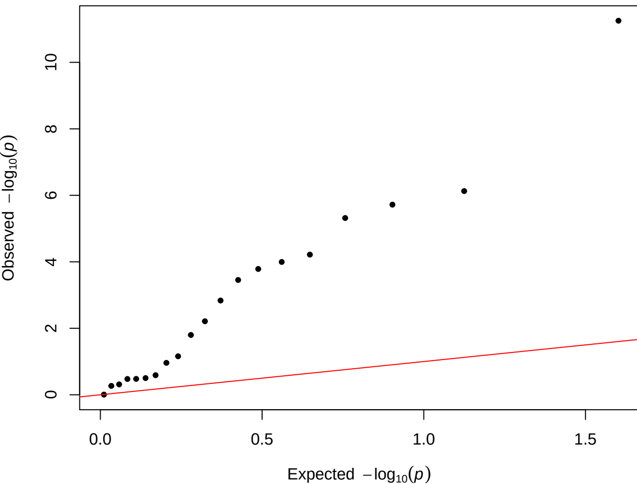
QQ Plot – all, FU=2, filtered
