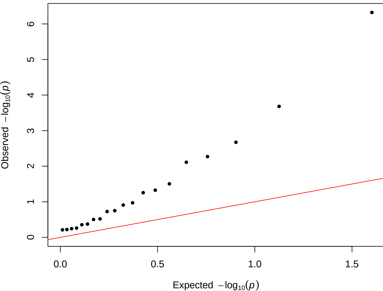
QQ Plot – male, FU=1, filtered
