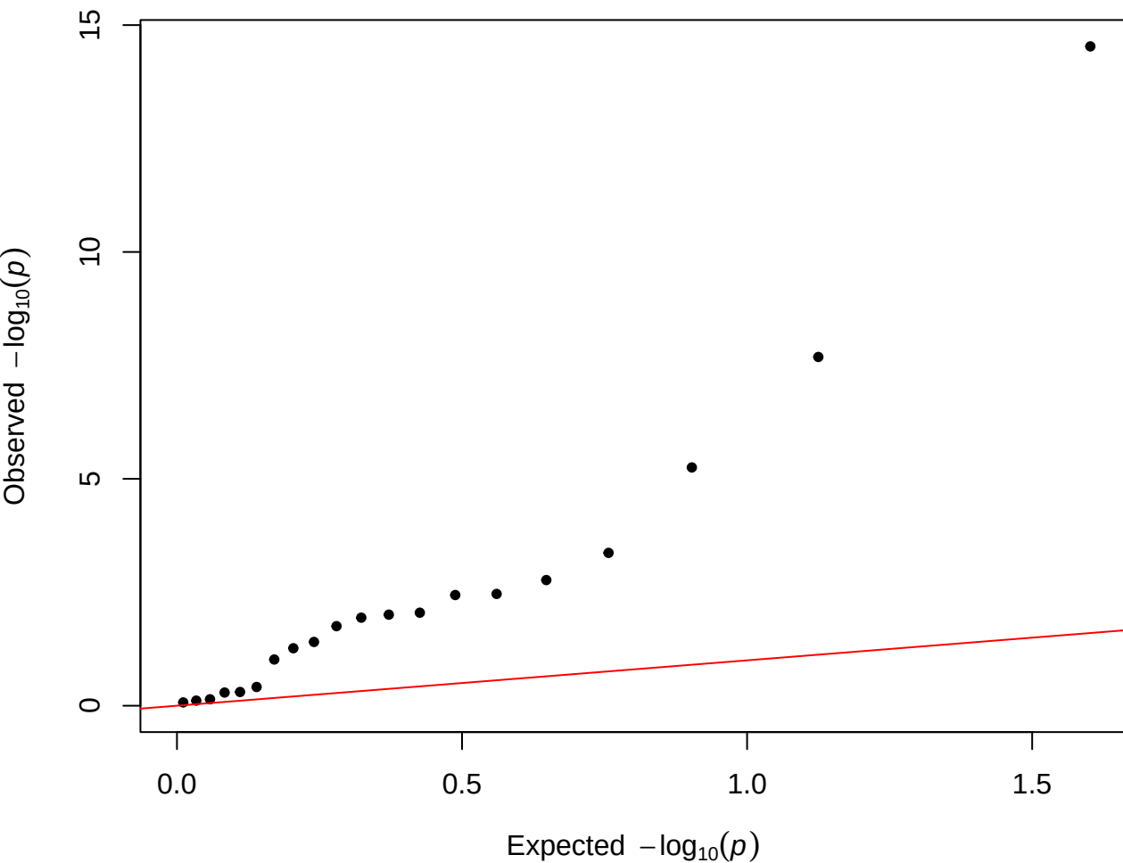
QQ Plot – all, FU=1, filtered
