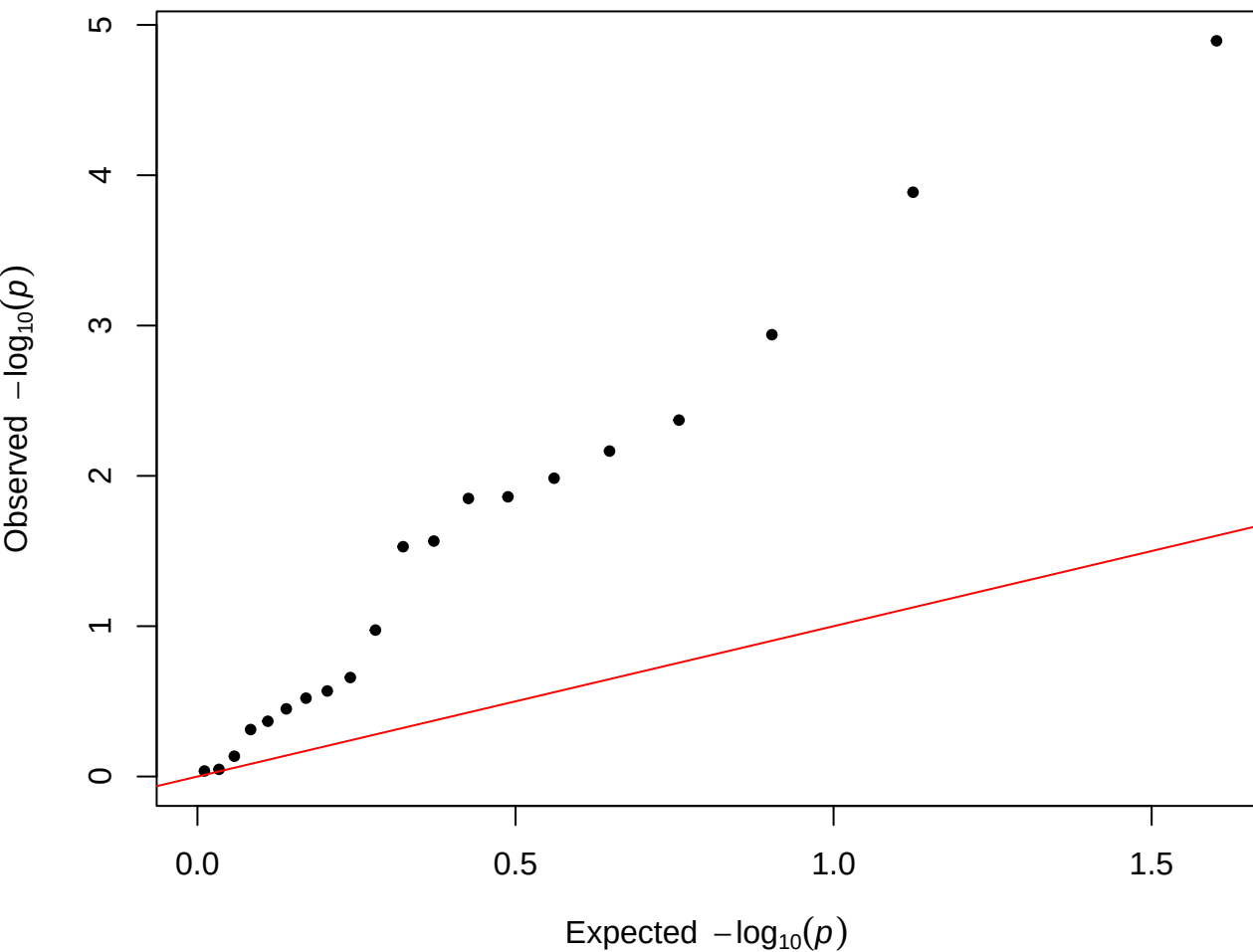
QQ Plot – male, FU=2, filtered
