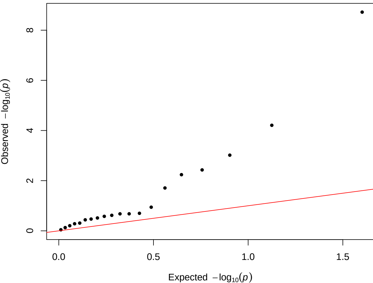
QQ Plot – female, FU=1, filtered
