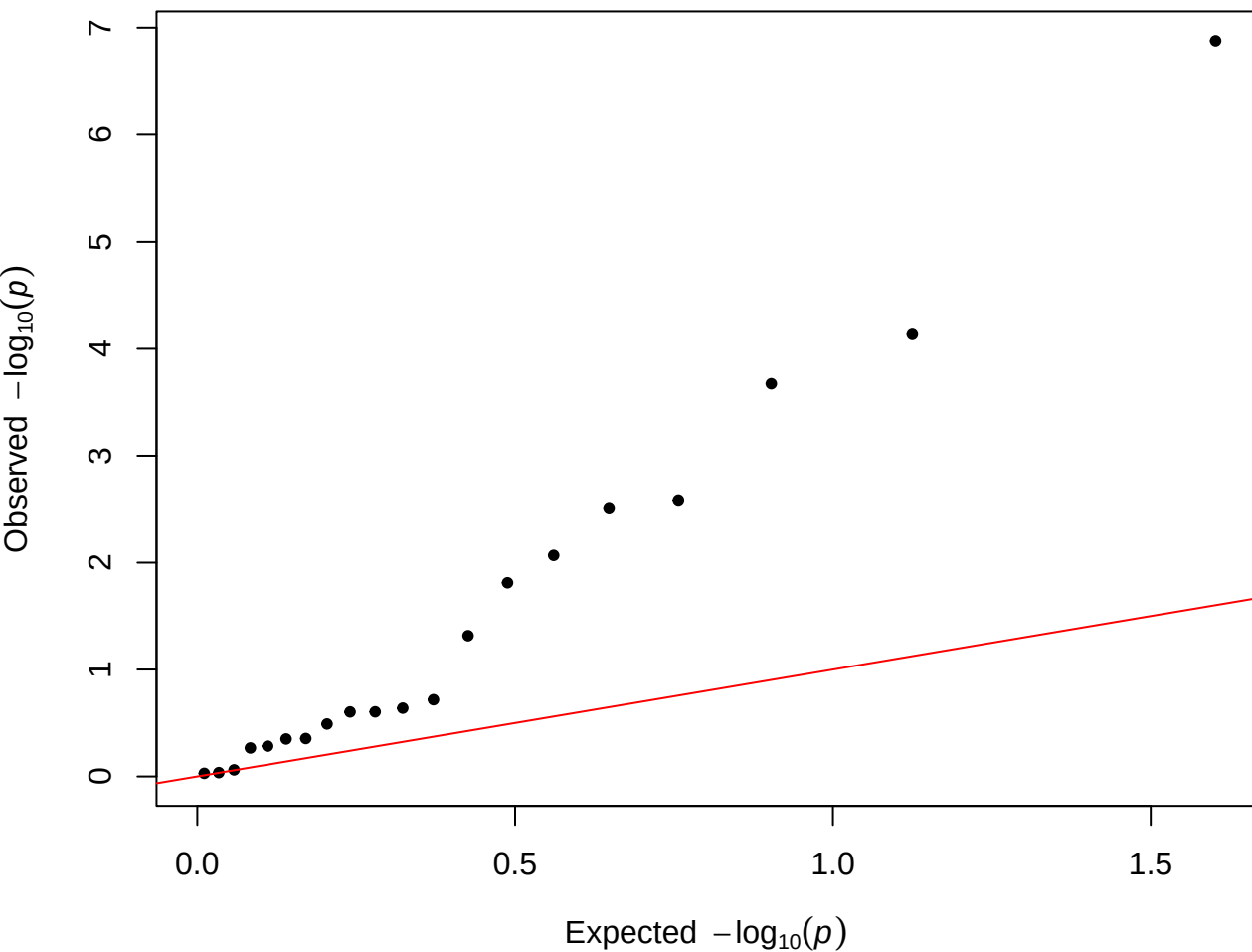
QQ Plot – female, FU=2, filtered
