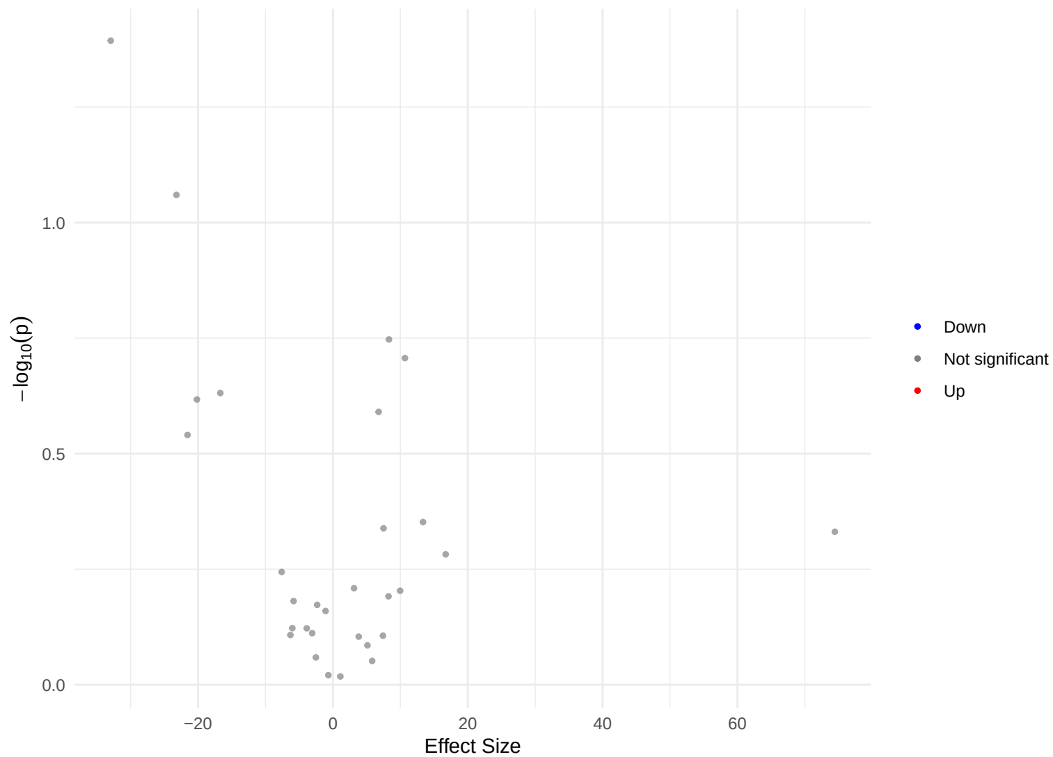
Volcano Plot – male, FU=2, full
