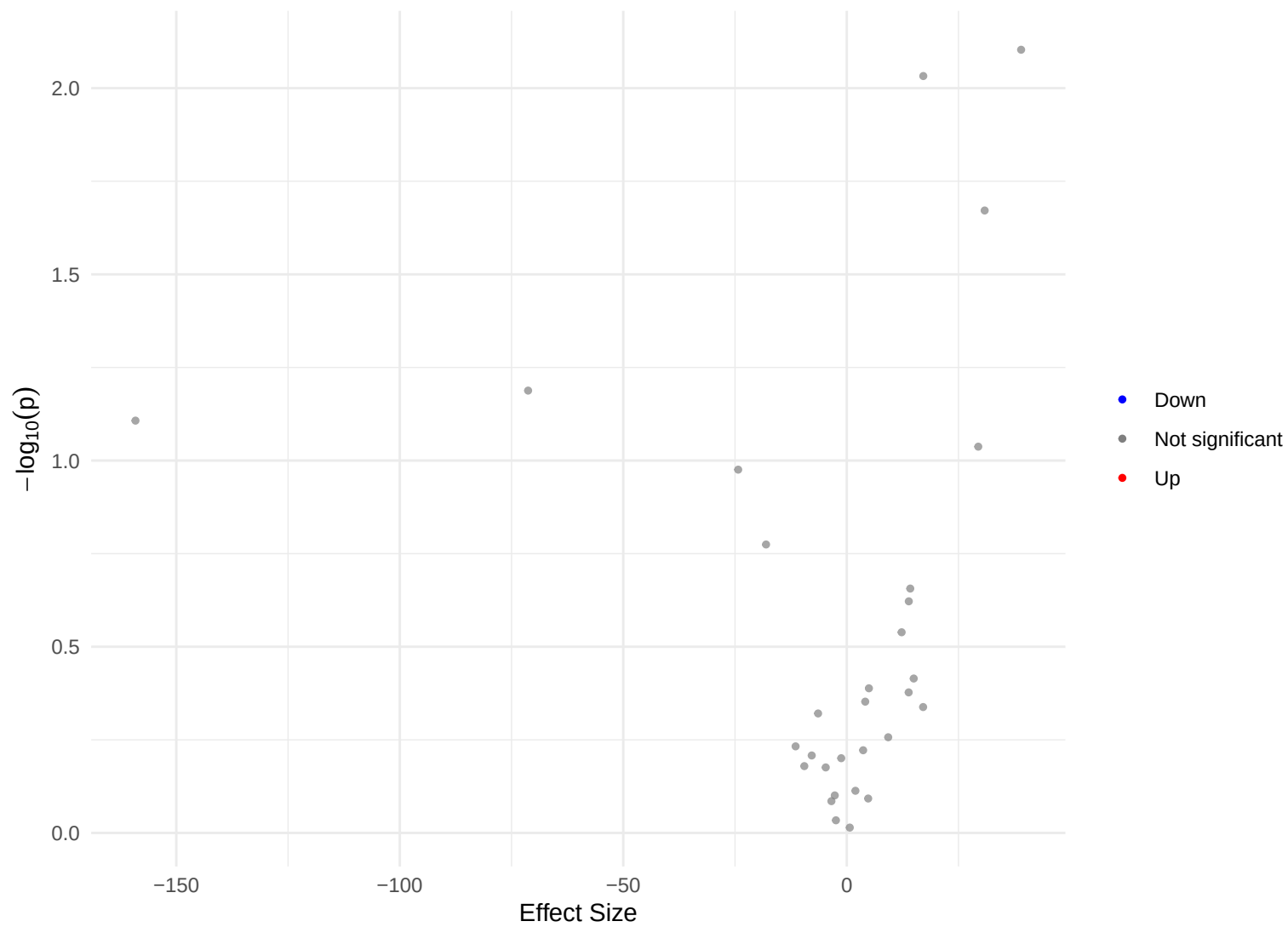
Volcano Plot – male, FU=1, full
