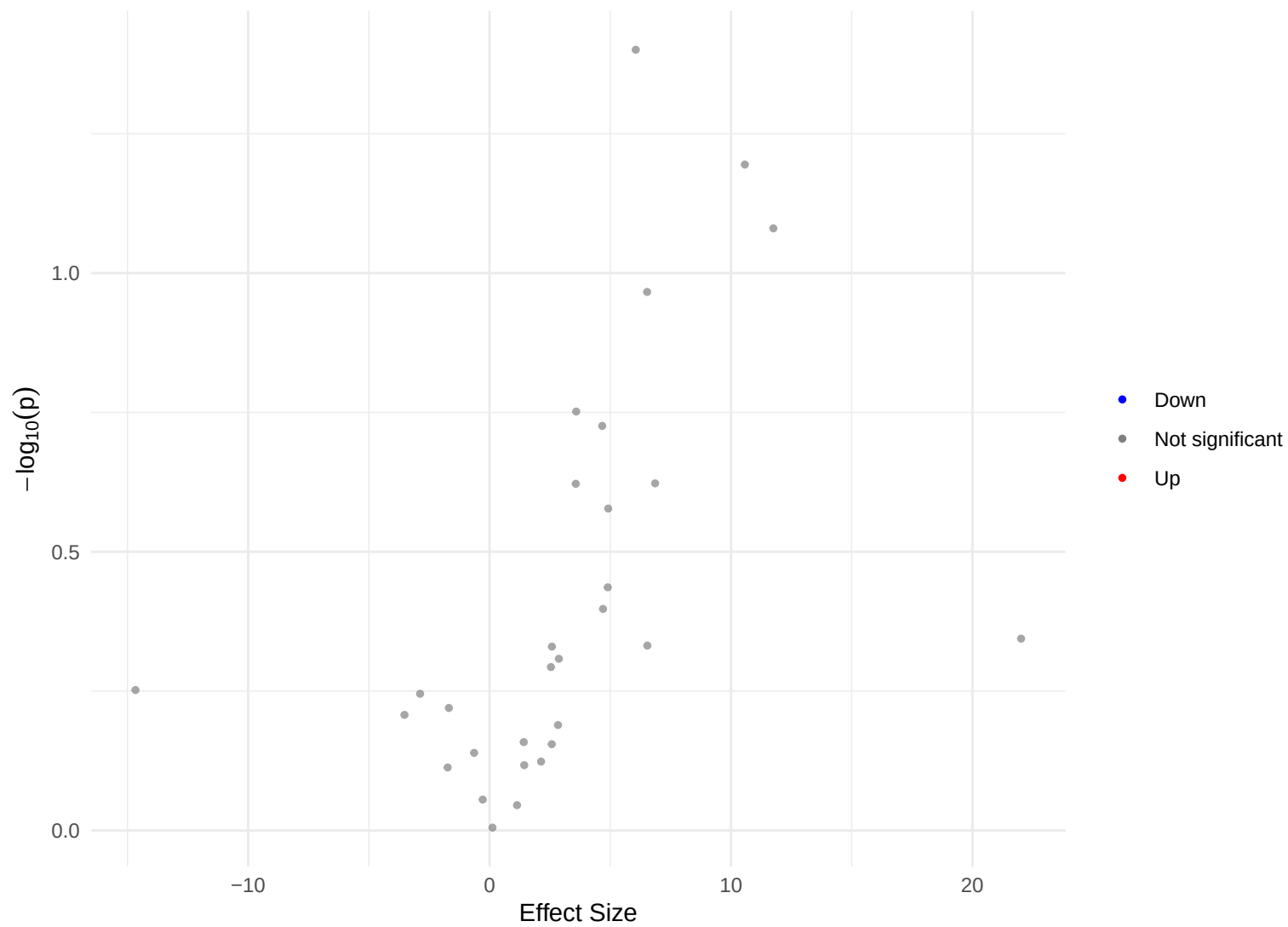
Volcano Plot – all, FU=2, full
