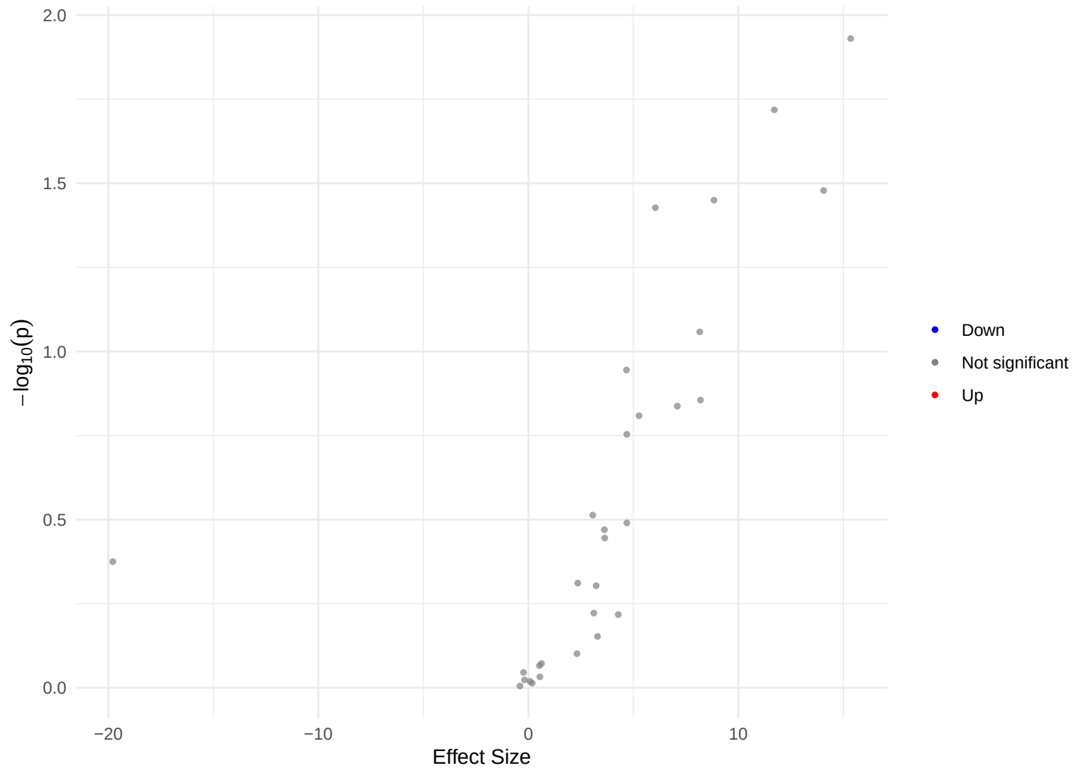
Volcano Plot – all, FU=1, full
