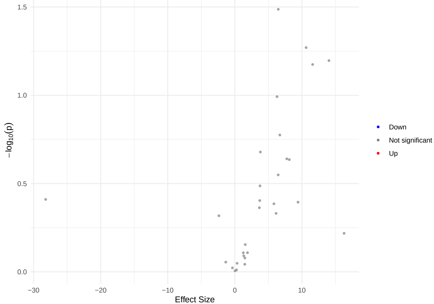
Volcano Plot – female, FU=2, full
