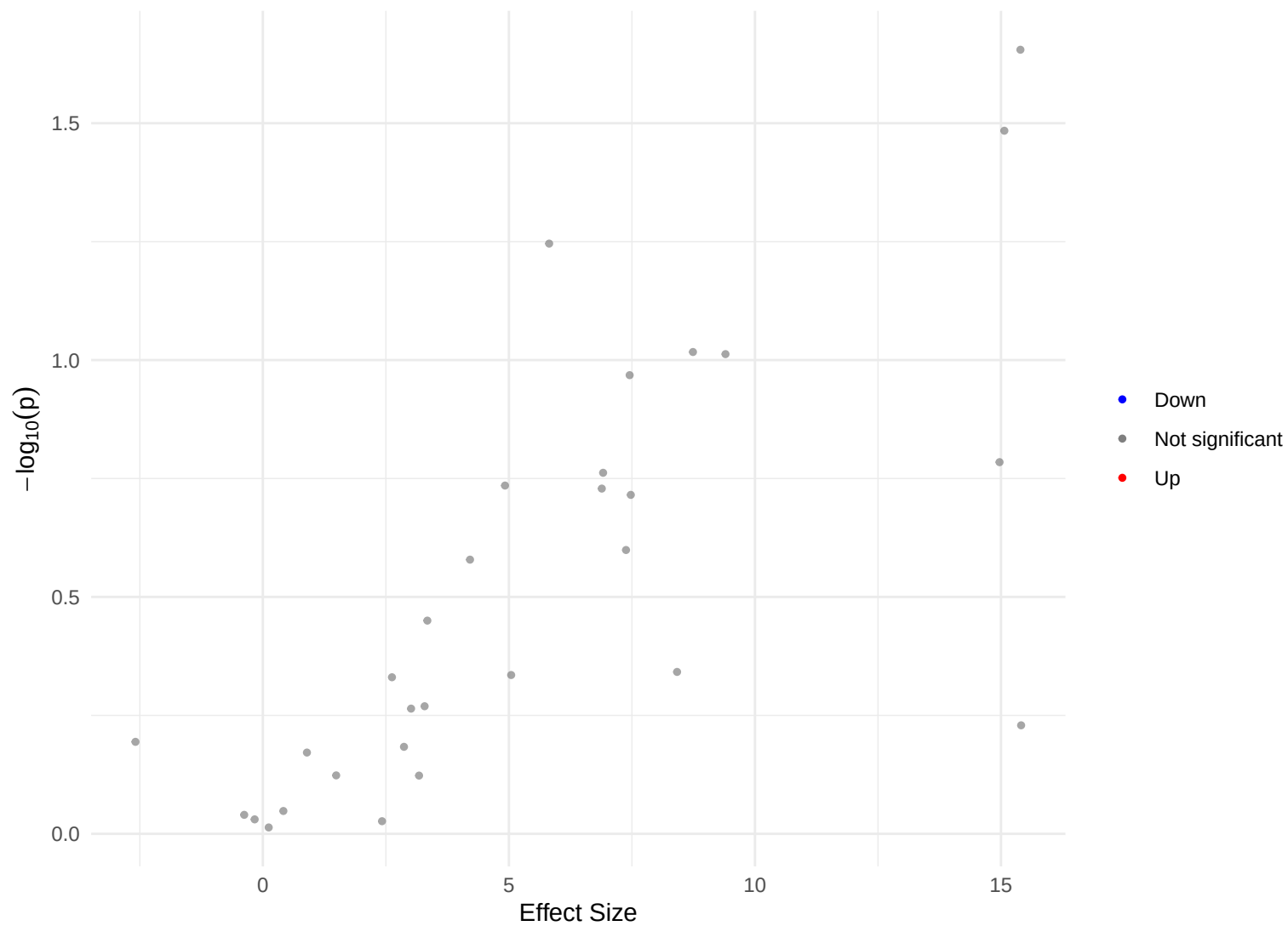
Volcano Plot – female, FU=1, full
