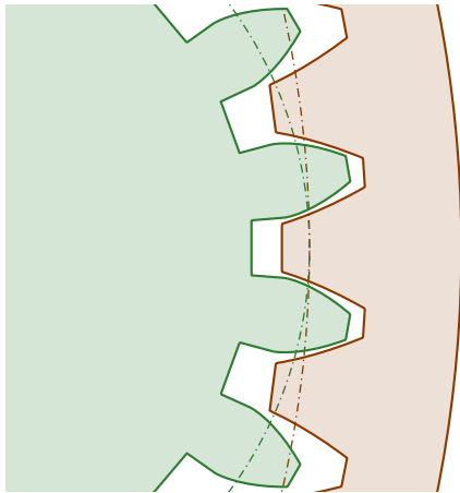
(b) engrenamento planeta-anel
