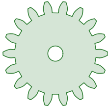
planeta (x3)
