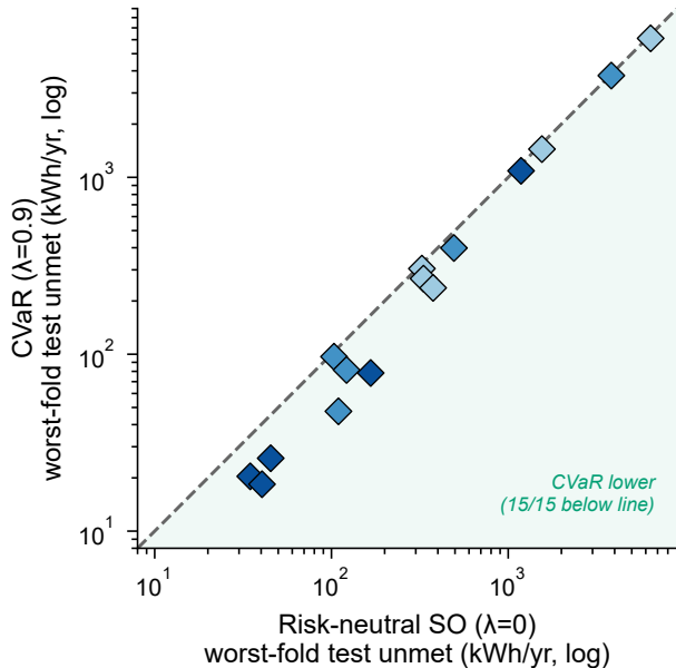
(b) Reliability tail
