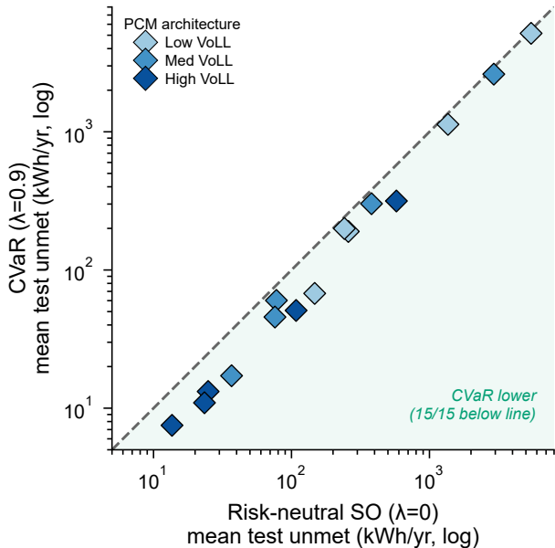
(a) Expected reliability
