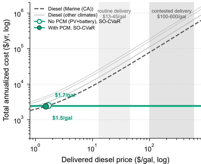
(a) Cost vs fuel price — Marine (CA)
