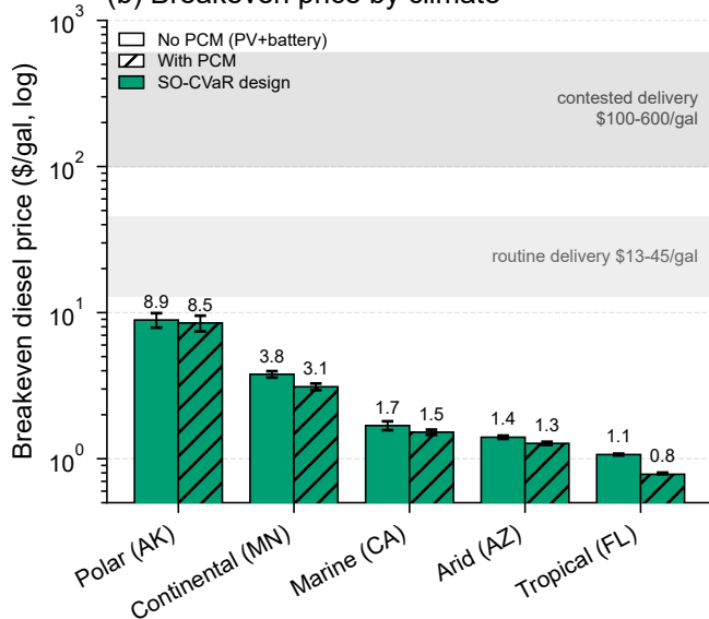
(b) Breakeven price by climate
