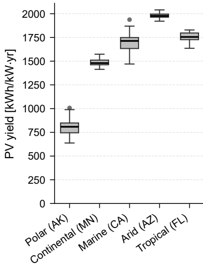
(a) Annual PV yield
