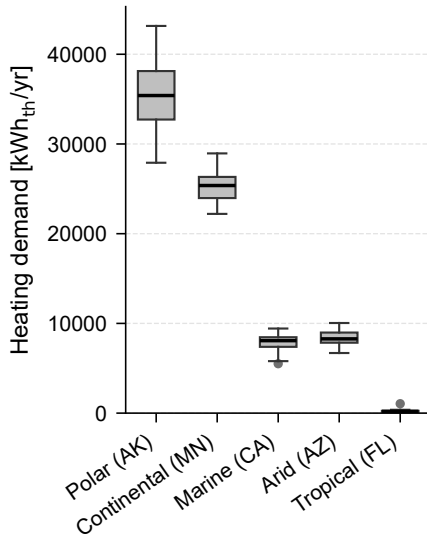
(b) Annual heating demand
