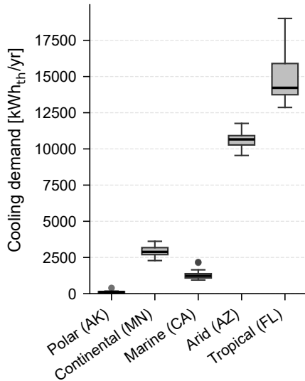
(c) Annual cooling demand
