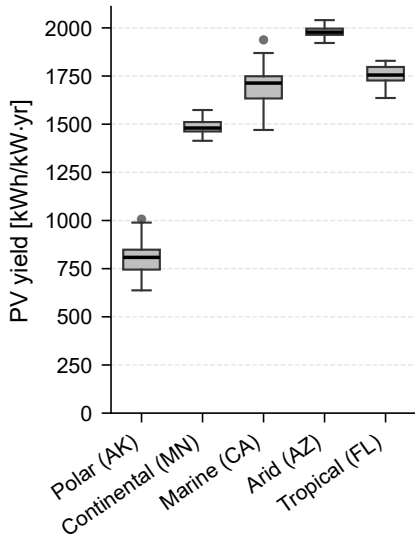
(a) Annual PV yield
