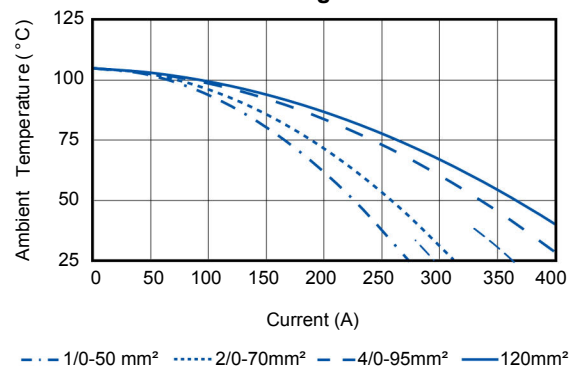
A320 Derating Curve 1
