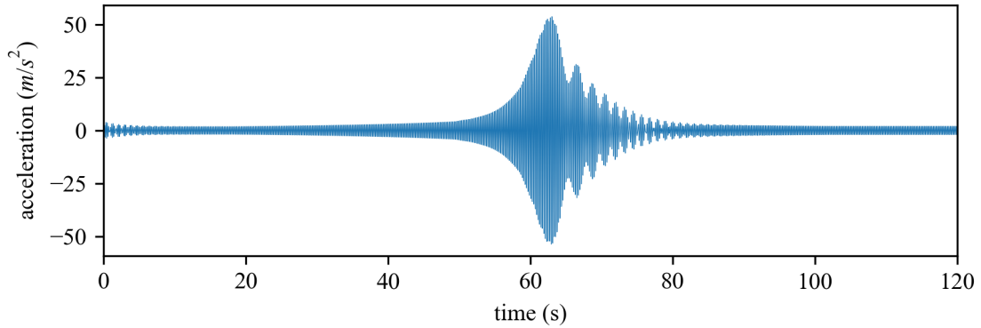
Figure 2: Measured acceleration for one test.
