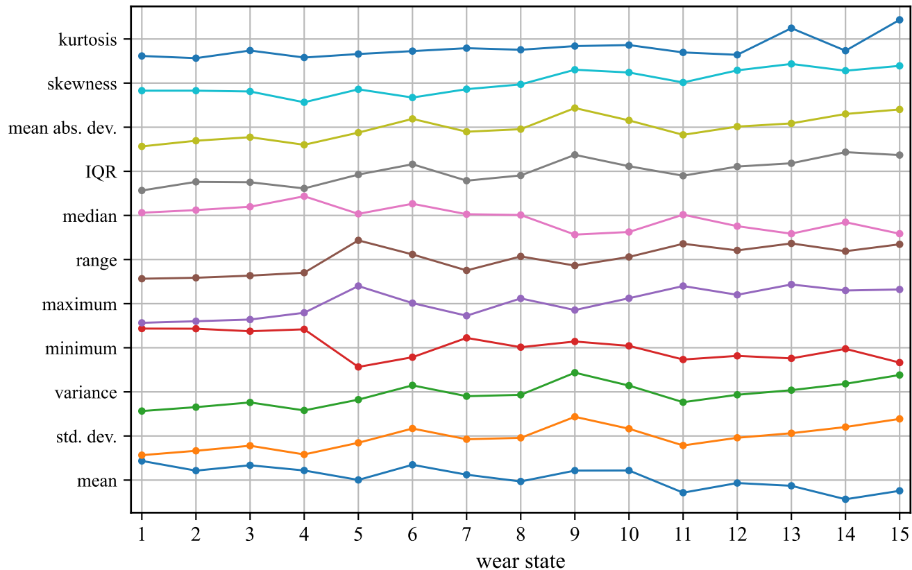
normalized feature traces for motor
