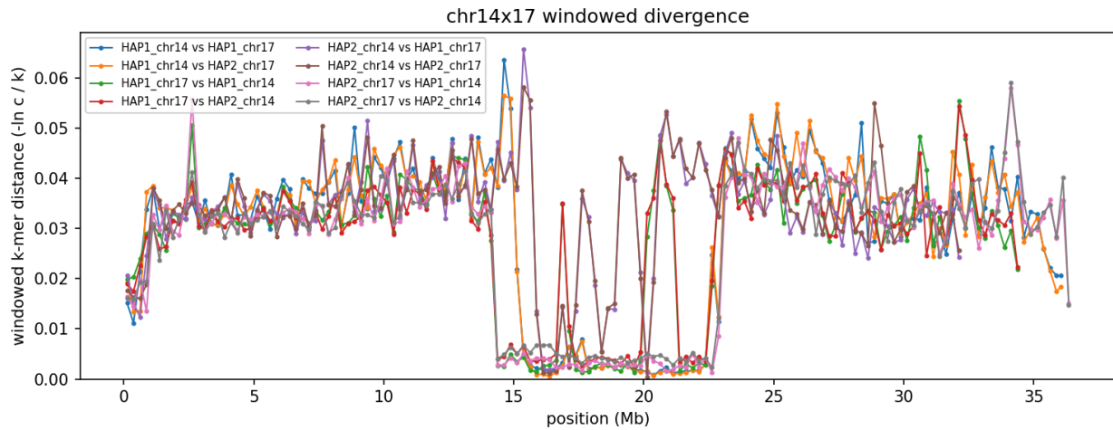
Figure 3: chr14 × chr17, all eight copy directions. Outside 14–23 Mb the homeologs are 0.03–0.05 apart; inside they drop to 0.003, as close as alleles. A mid-chromosome block like this could be retained pairing, a recent homeologous exchange shared by both haplotypes, or a centromeric repeat specific to this pair: the data cannot tell which.
