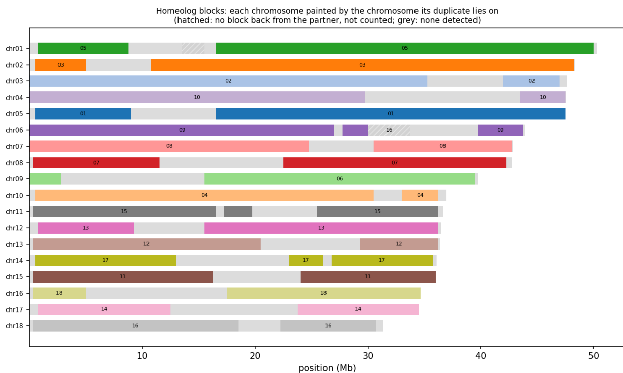
Figure 2: Glechoma: every chromosome is duplicated on exactly one partner along most of its length. Grey gaps are regions where the homeolog is not detected (diverged beyond k-mer reach, or lost).
