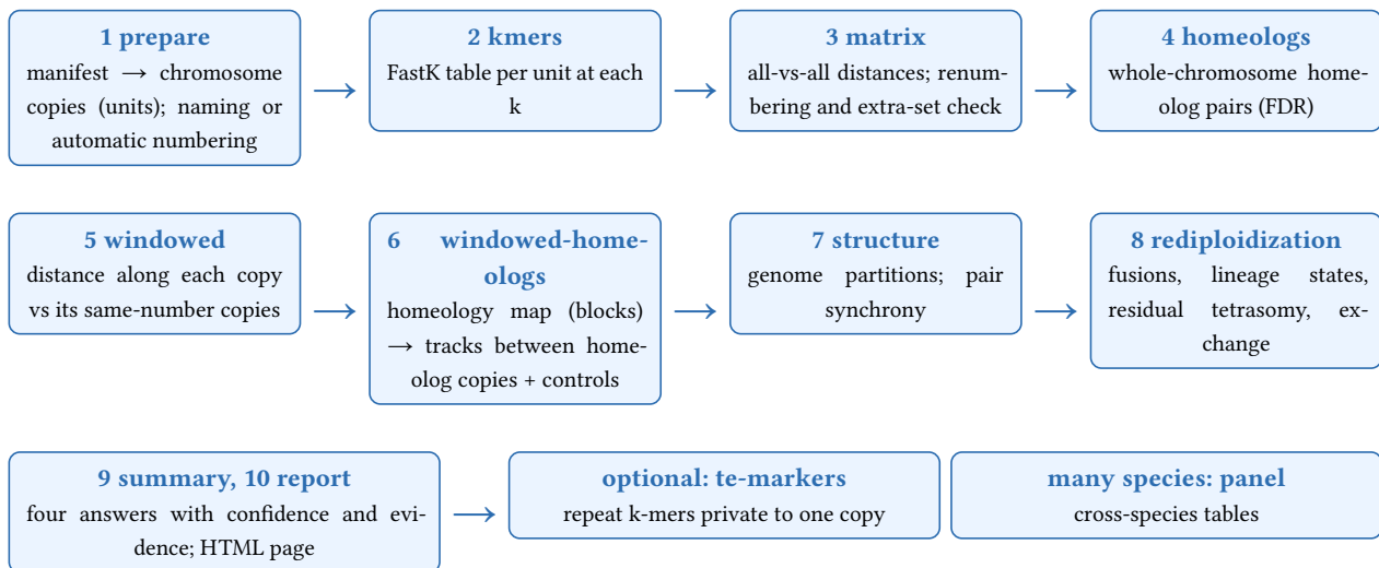
Figure 1: ploidyspec all runs these in order. Stage 6 runs with --with-windowed-homeologs (recommended), te-markers with --with-te-markers . Each stage reads only files written by earlier stages, so any stage can be re-run on its own.
