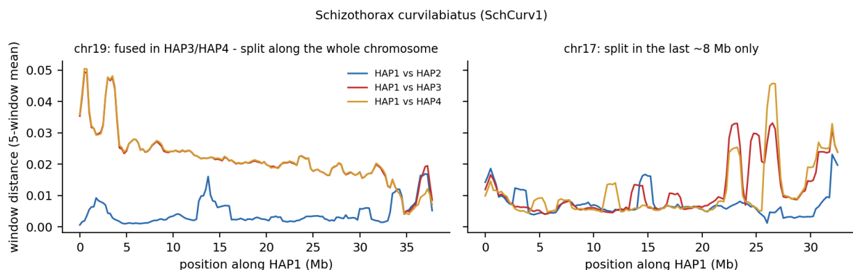
Figure 4: SchCurv1 windows along HAP1. chr19: the fused copies stay far all along. chr17: the copies separate only towards the end.
