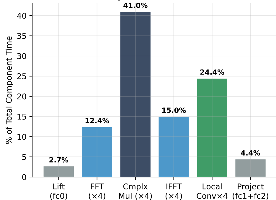
FNO Component Time Breakdown
