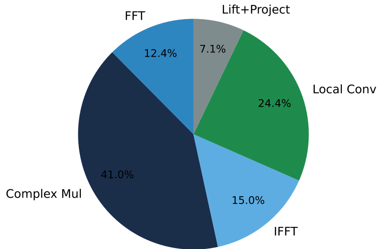
Spectral ops = 68.4% of compute
