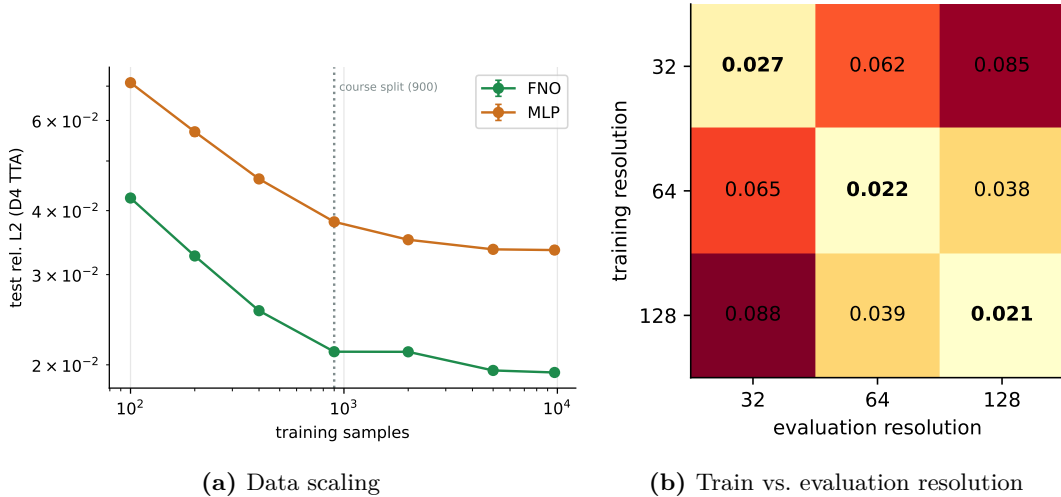
Figure 3: (a) FNO error falls from 0.042 ( n = 100 ) to 0.0195 ( n = 5000 ) and then saturates; at 200 samples the FNO is at 0.033 vs. 0.057 for the MLP, which plateaus at 0.034. (b) Test error of FNOs trained at one resolution and evaluated at another (2 seeds).
