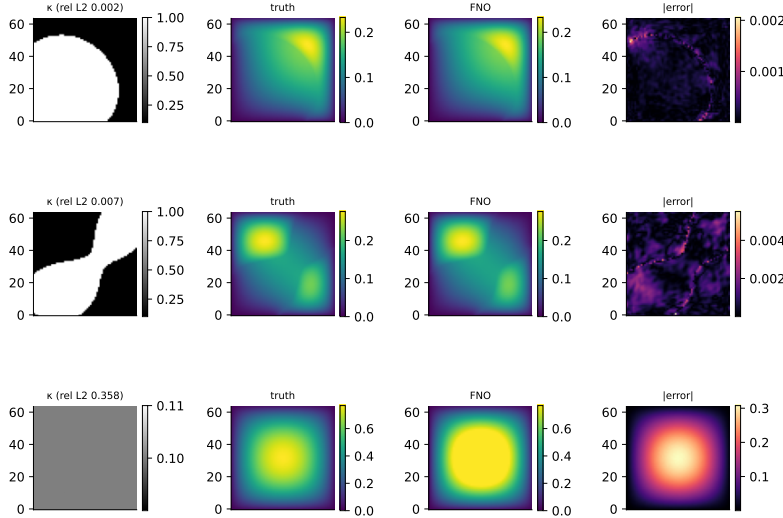
Figure 6: Best, median and worst test sample of the final FNO: \kappa (relative error in title), truth, prediction, absolute error. The worst case has uniform \kappa = 0.1 .
