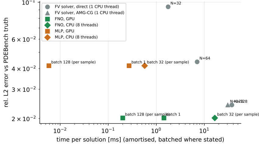
Figure 4: Error-time trade-off. Solver: 1 CPU thread. FNO/MLP: GPU or 8-thread CPU as marked.
