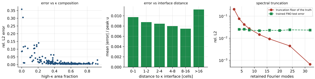
Figure 5: Left: error vs. high-permeability area fraction. Middle: mean absolute error (relative to the field’s peak pressure) vs. distance to the nearest \kappa interface. Right: relative error of the truth when truncated to m Fourier modes (red) vs. the test error of FNOs actually trained with m modes (green).
