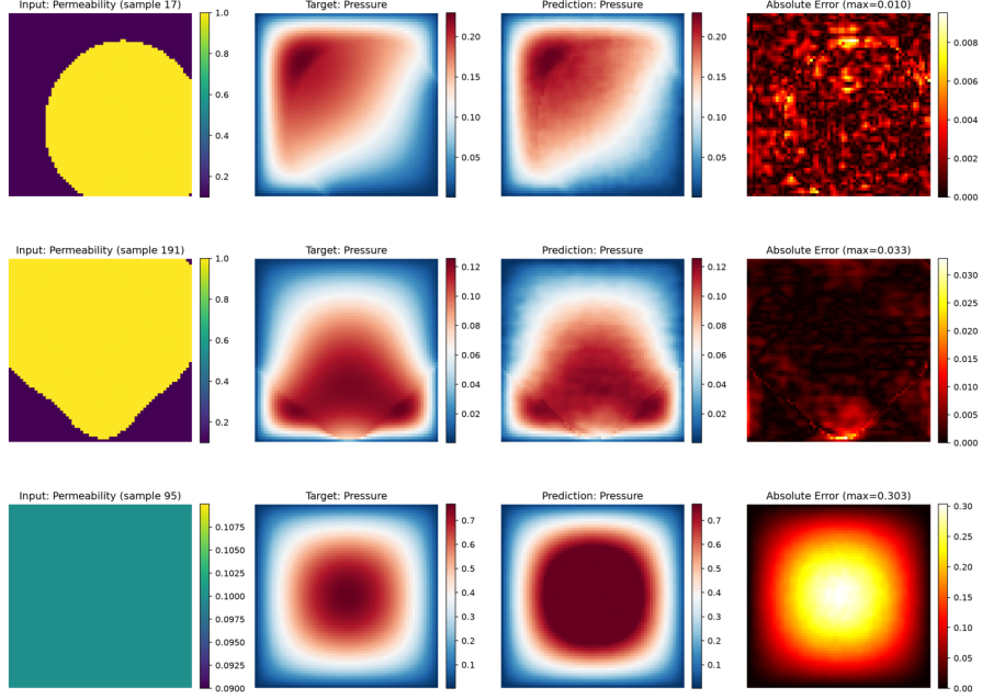
Figure 6: FNO predictions for the best (sample 17, error 0.016), a median-error (sample 191, error 0.040) and the worst (sample 95, error 0.347) test sample. Columns: input \kappa , target pressure, predicted pressure, absolute error. The worst case has exactly uniform \kappa \equiv 0.1 : the true pressure is a smooth bump, but the FNO over-predicts its amplitude (the prediction saturates the colour scale of the target), a failure mode specific to this degenerate input.
