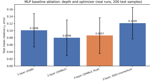
Figure 4: MLP baseline ablation (error bars: one standard deviation across the 200 test samples).
