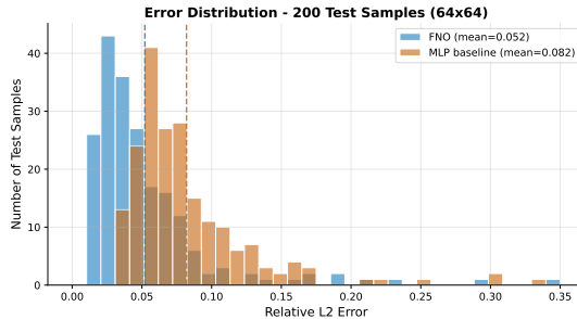
Figure 5: Error distribution across 200 test samples. Dashed vertical lines indicate per-model means. FNO errors are concentrated at lower values; the MLP’s distribution is shifted right.
