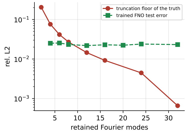
spectral truncation
