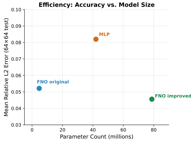
Figure 3: Accuracy–parameter efficiency. FNO original occupies the optimal region: 9\times fewer parameters than MLP at 37% lower error. Scaling FNO to 78.8M yields only 12% further improvement.
