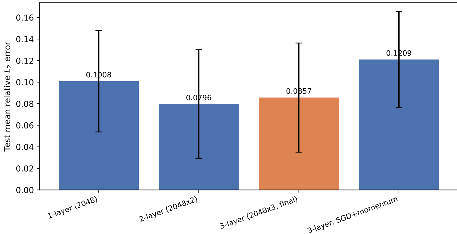
MLP baseline ablation: depth and optimizer (real runs, 200 test samples)
