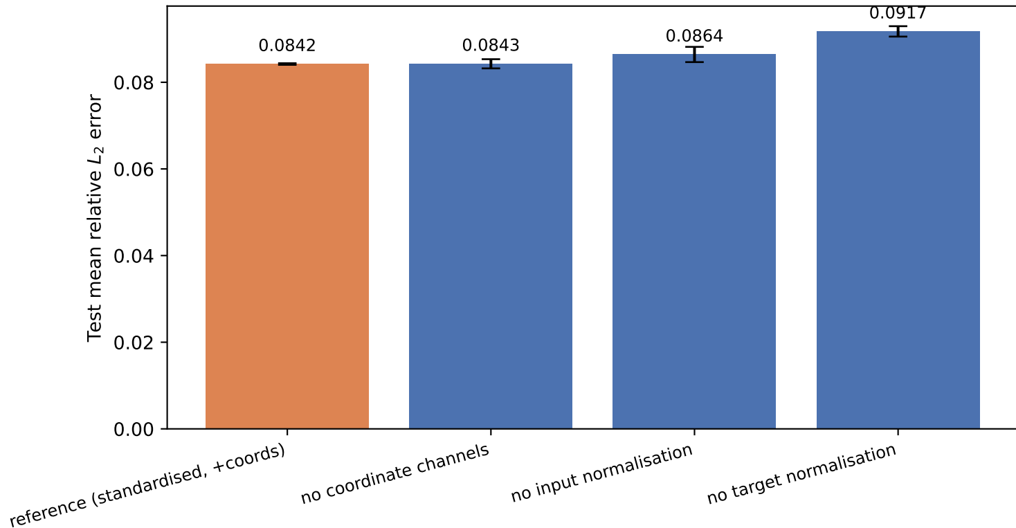
MLP preprocessing ablation (mean \pm std over 3 seeds)
