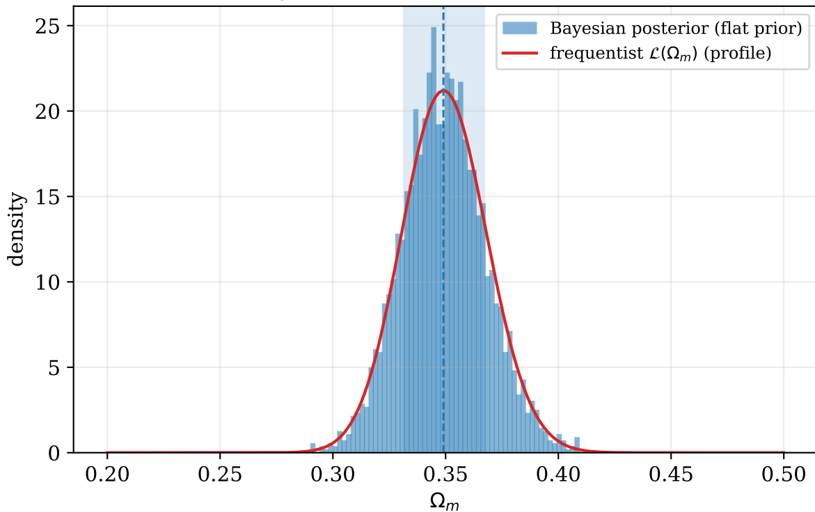
flat \Lambda CDM: Bayesian posterior vs frequentist likelihood
