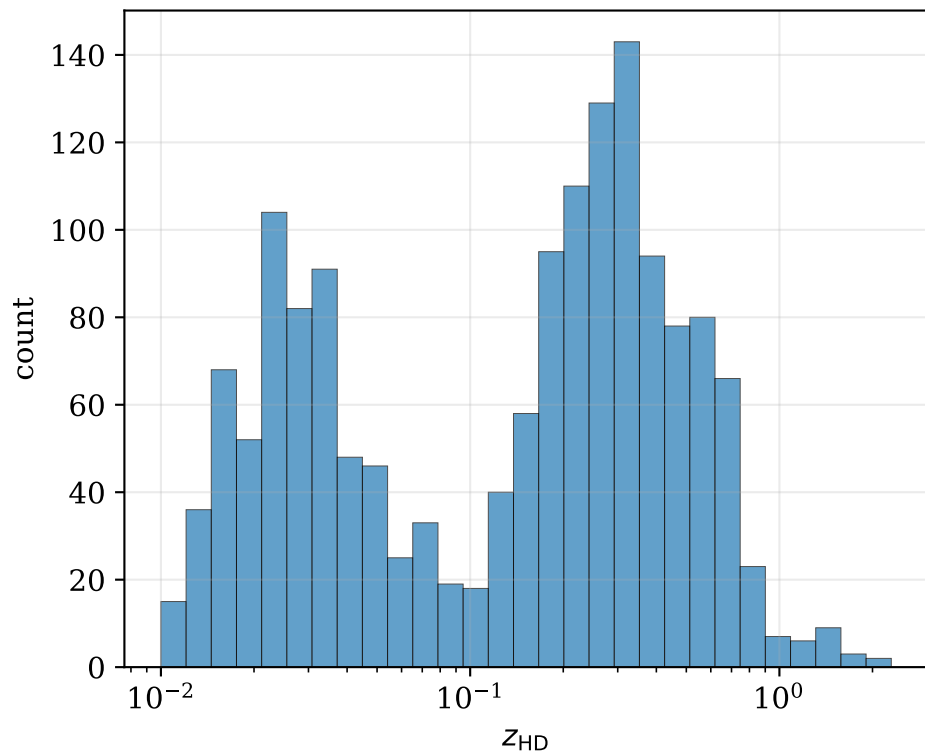
Redshift distribution
