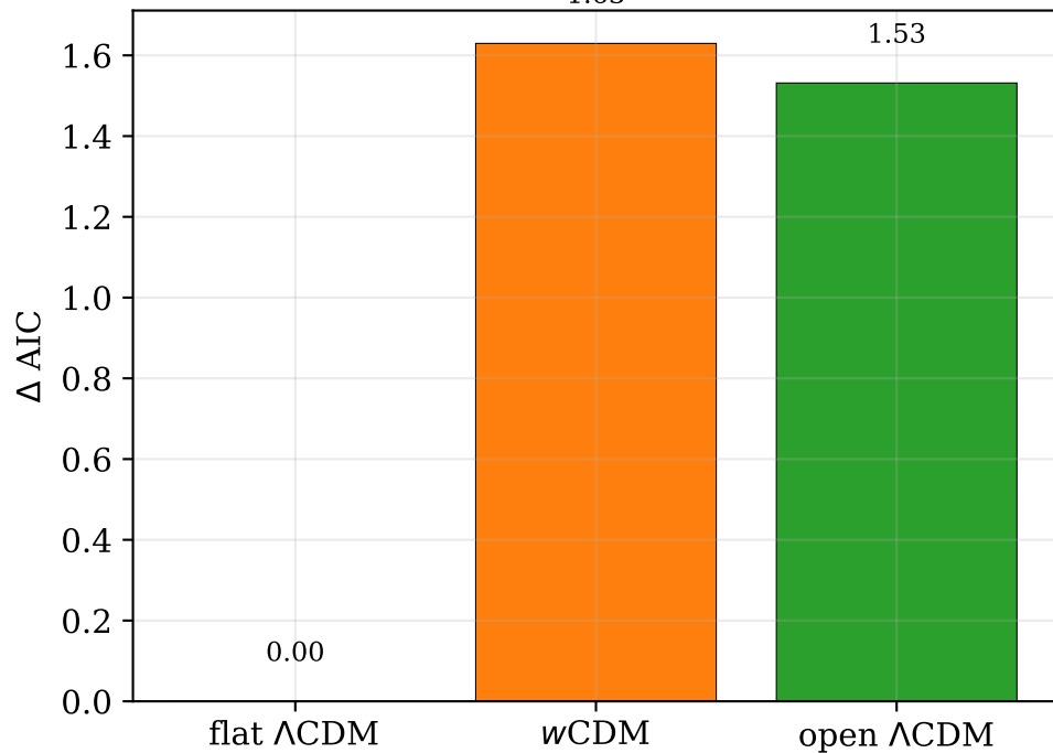
Akaike information criterion
