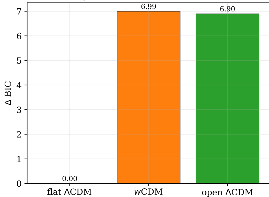
Bayesian information criterion
