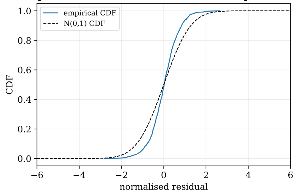
Empirical CDF vs N(0,1), KS D = 0.131, p = 2.8e-24
