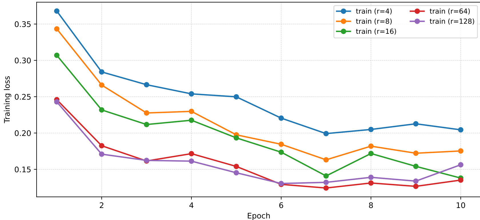
SST-2: rSVD Weight Reduction + SVT training loss vs epoch
