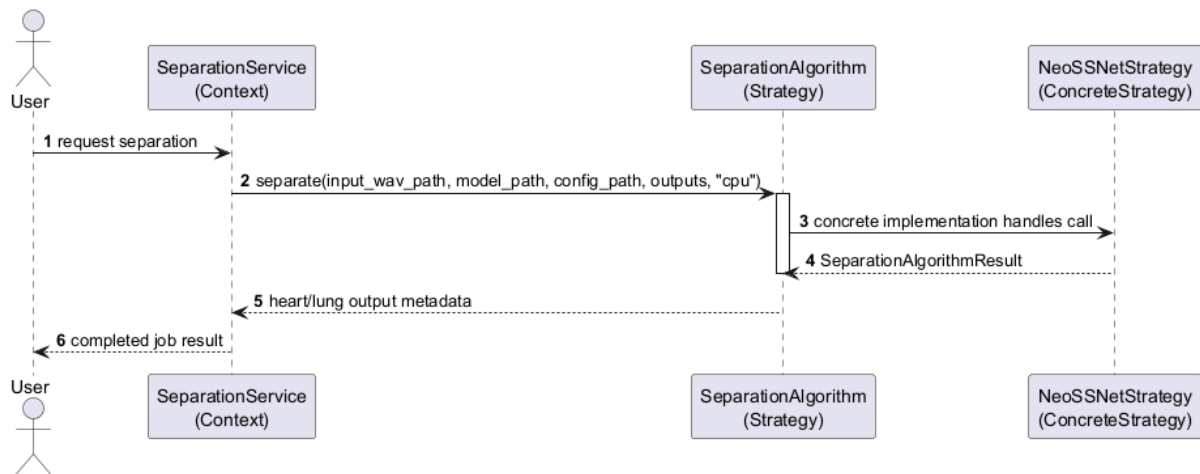
Figure 4.6: Strategy Pattern Sequence Diagram
