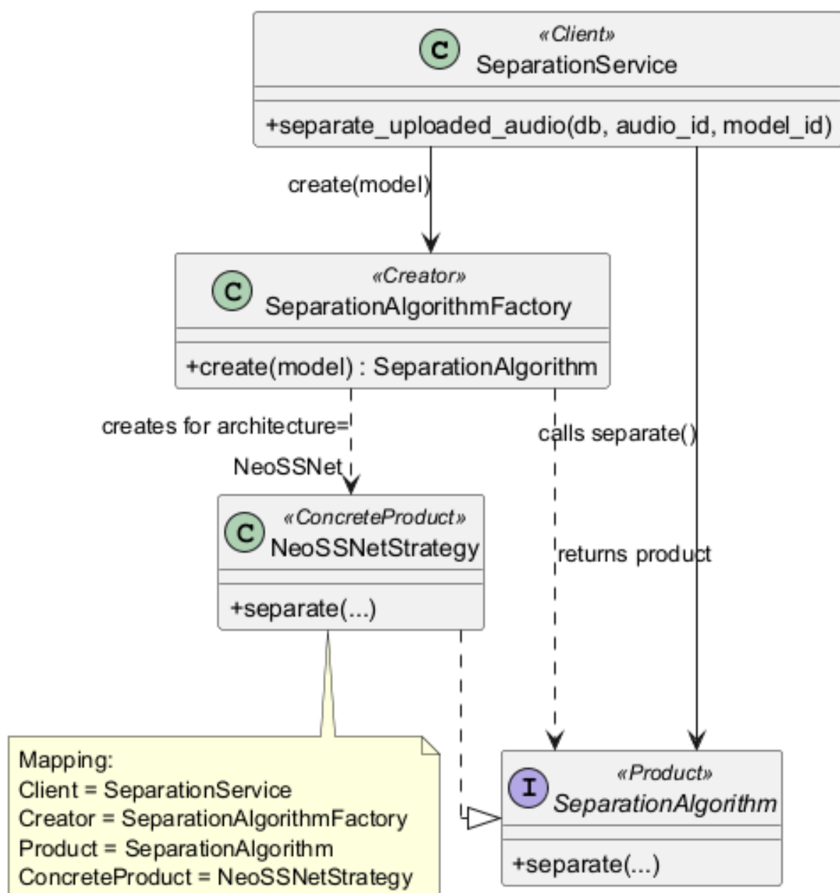
Figure 4.8: Factory Method Pattern Project Class Diagram
