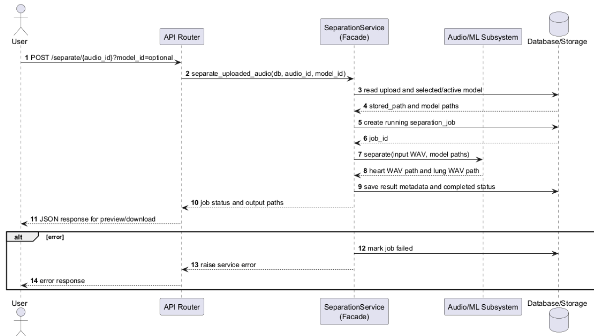
Figure 4.3: Facade Pattern Sequence Diagram
