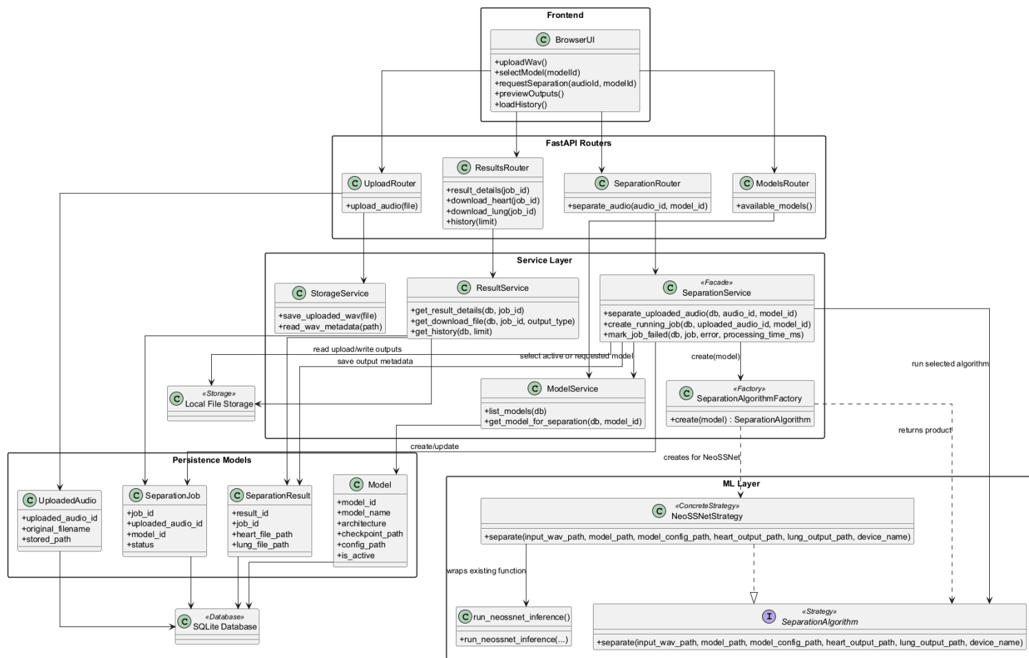
Figure 2.2: Overall System Class Diagram
