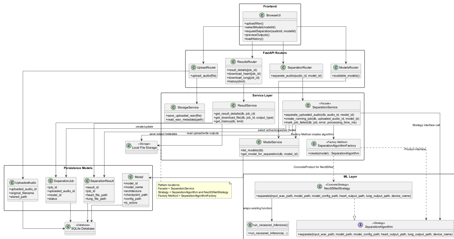
Figure 2.2: Overall System Class Diagram
