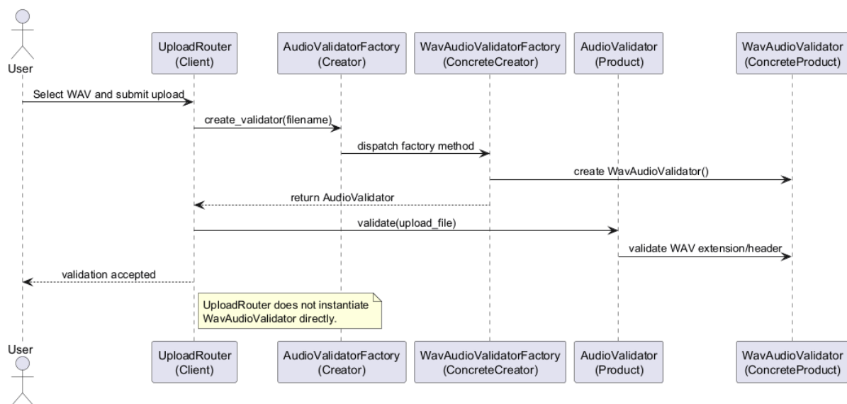
Figure 4.9: Factory Method Pattern Sequence Diagram
