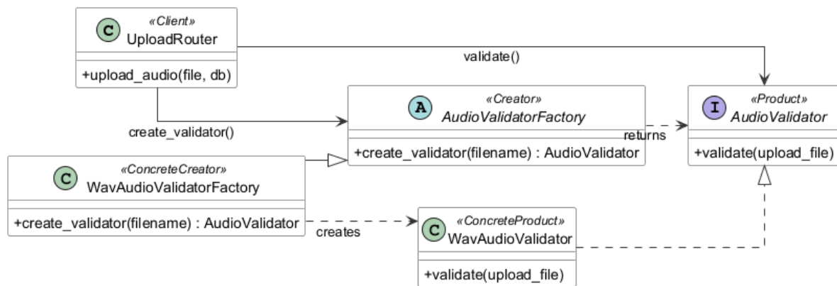
Figure 4.8: Factory Method Pattern Project Class Diagram
