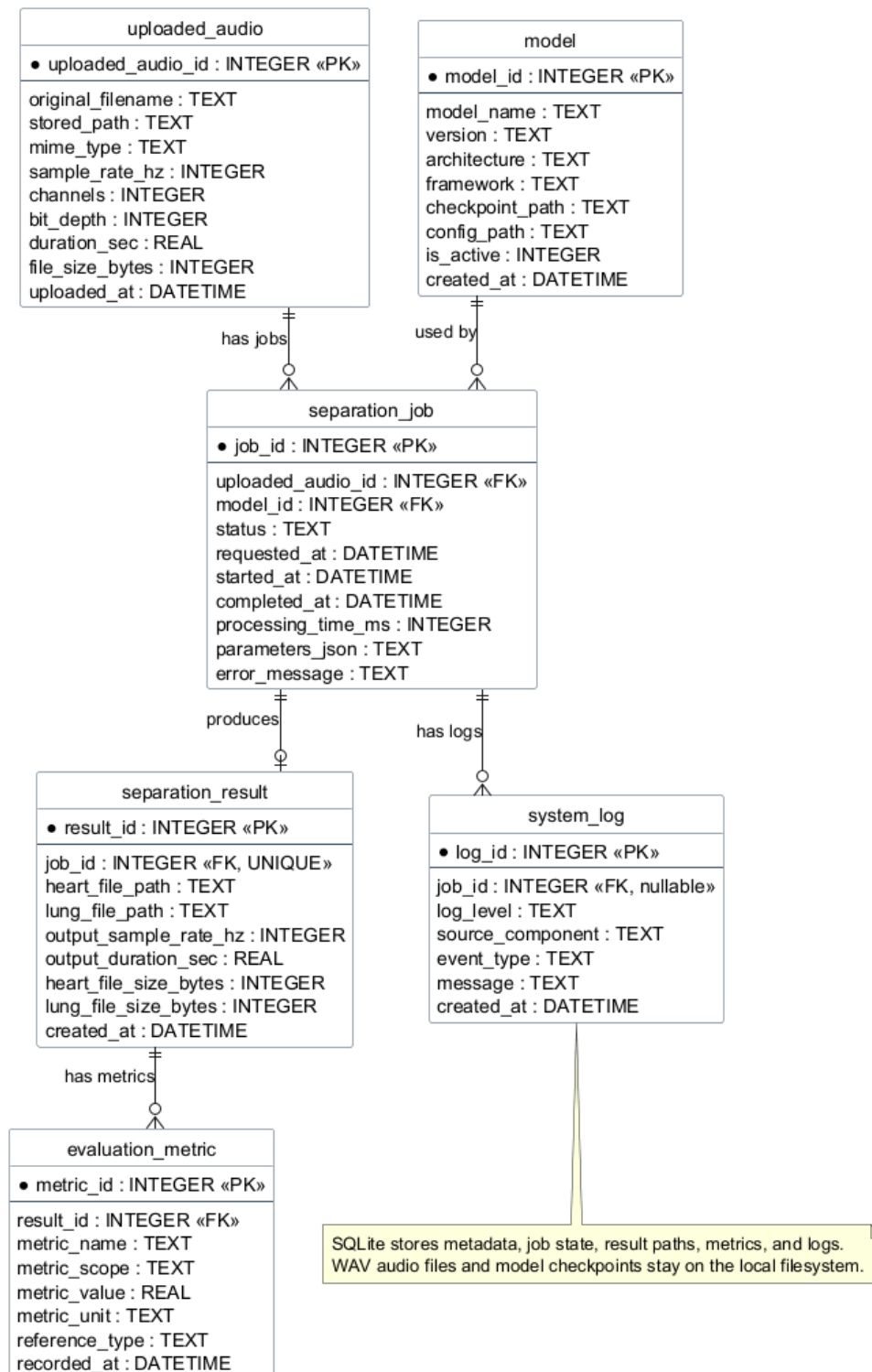
Figure 2.5: Entity Relationship Diagram
