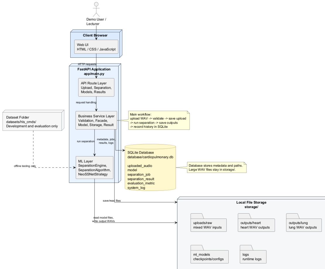
Figure 2.2: Software Architecture Diagram
