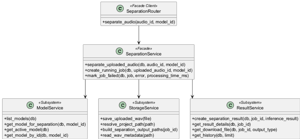
Figure 4.2: Facade Pattern Project Class Diagram
