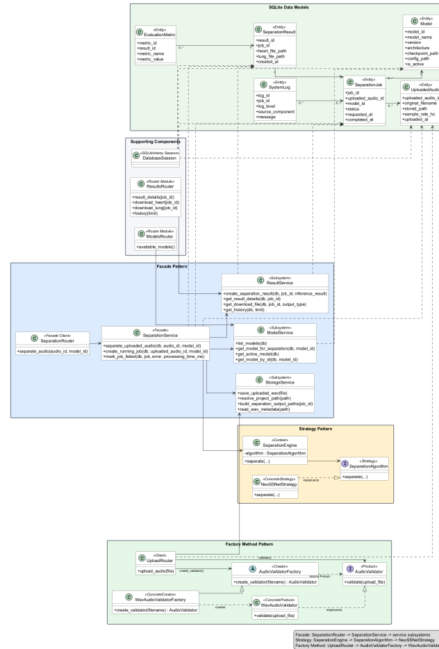
Figure 2.4: Overall System UML Class Diagram
