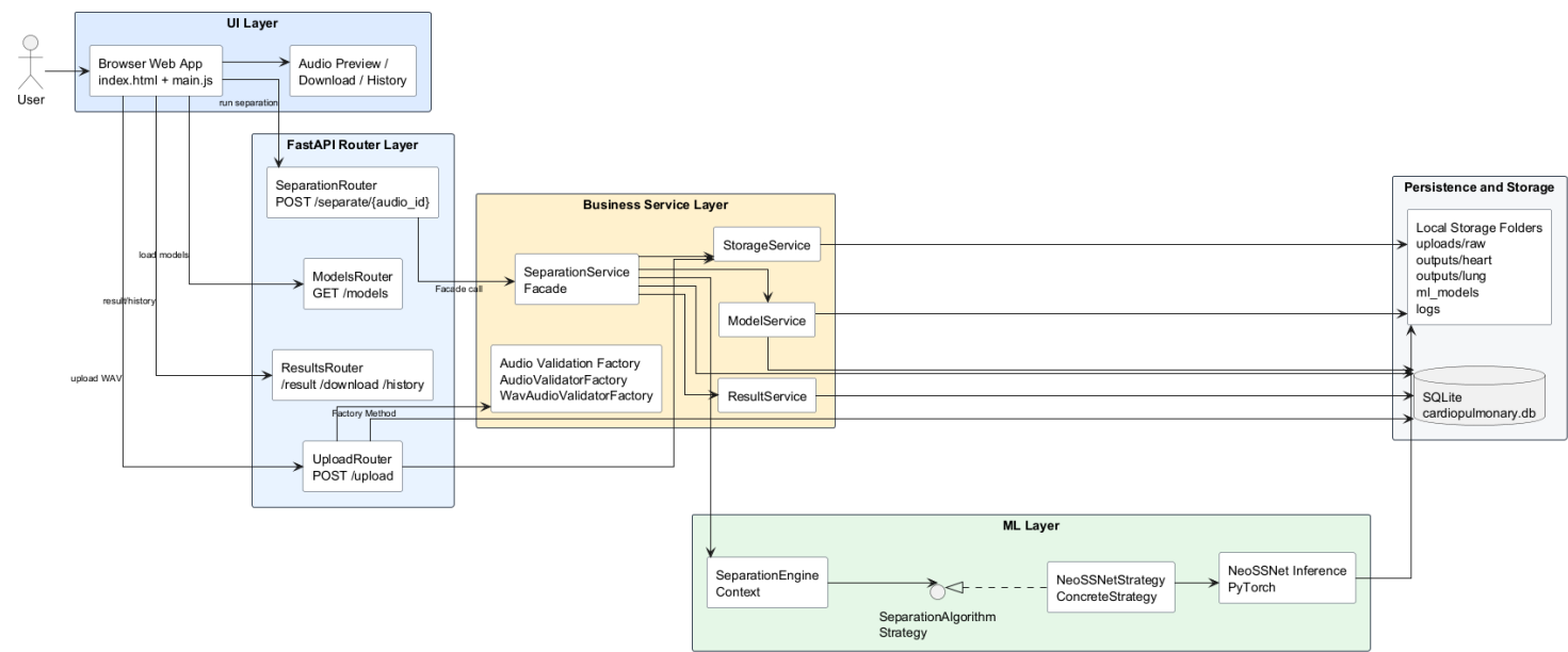
Figure 2.3: Component Level Diagram
