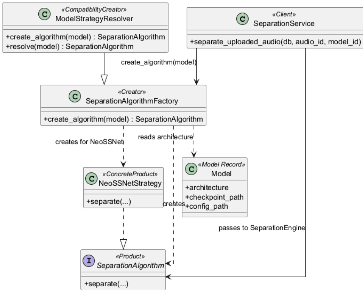
Figure 4.8: Factory Method Pattern Project Class Diagram
