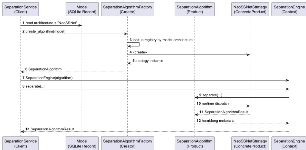
Figure 4.9: Factory Method Pattern Sequence Diagram
