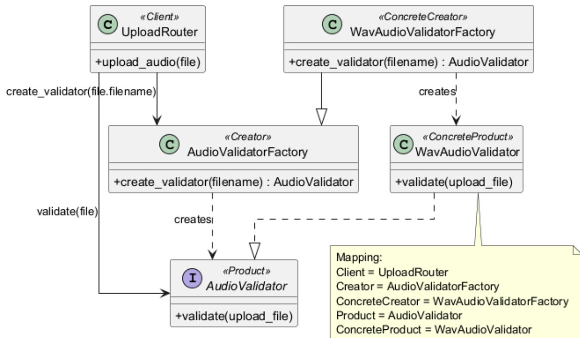
Figure 4.8: Factory Method Pattern Project Class Diagram
