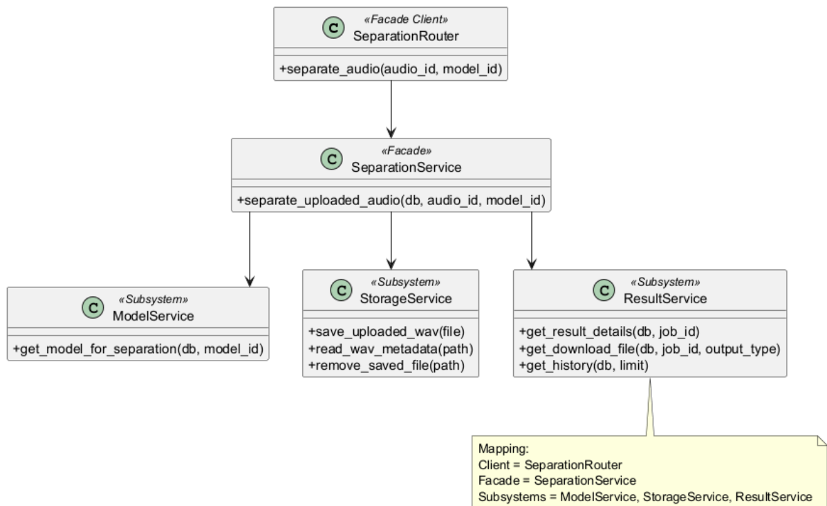
Figure 4.2: Facade Pattern Project Class Diagram
