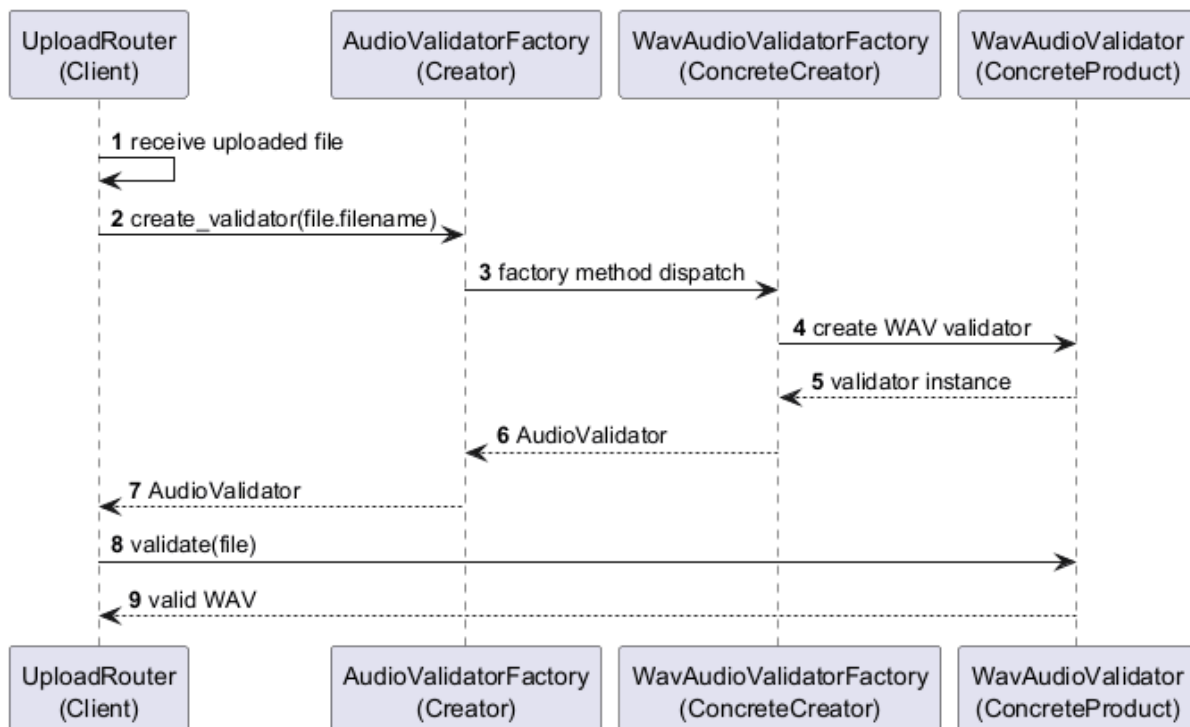
Figure 4.9: Factory Method Pattern Sequence Diagram
