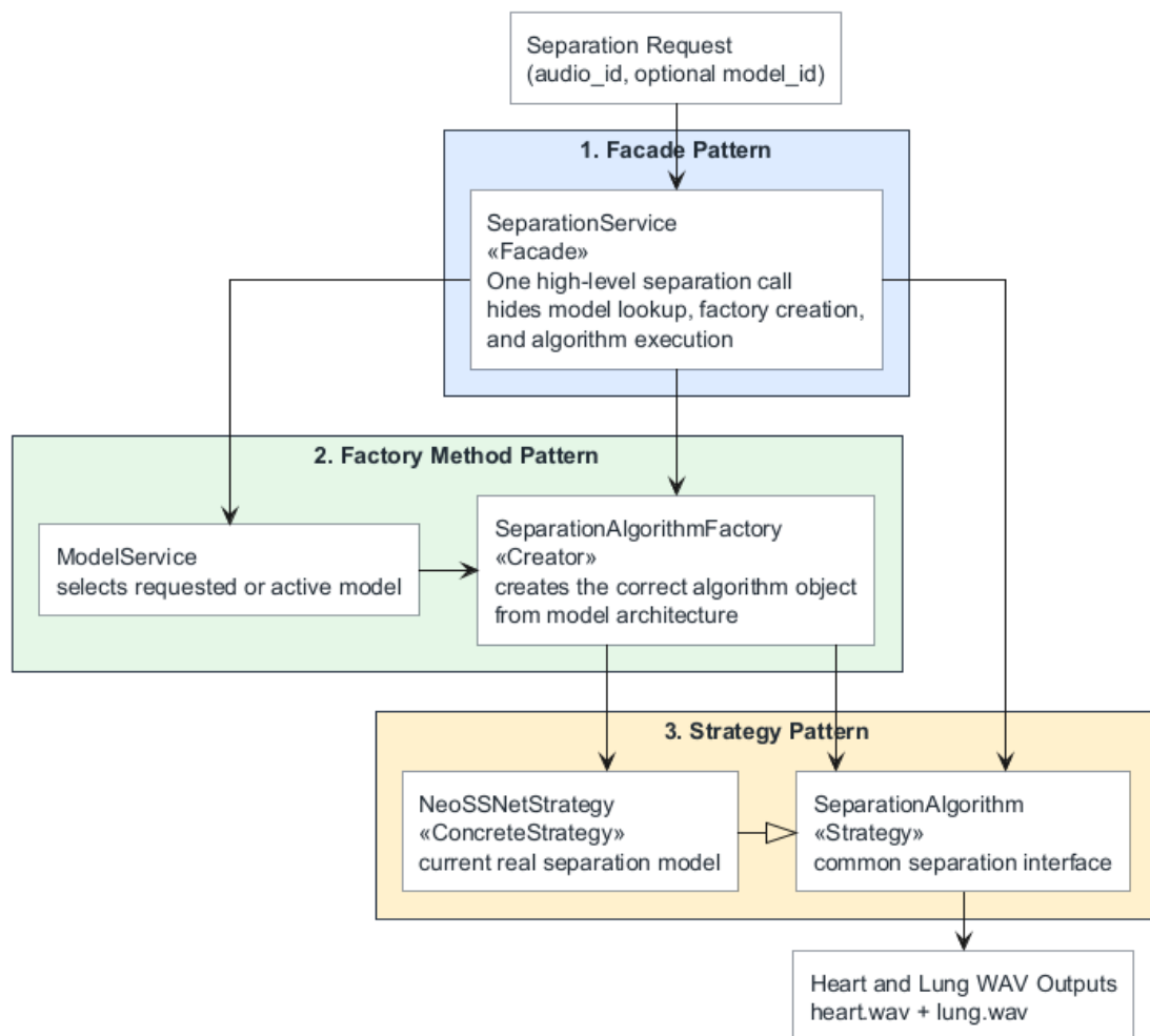
Figure 2.3: Design Pattern Location Overview
