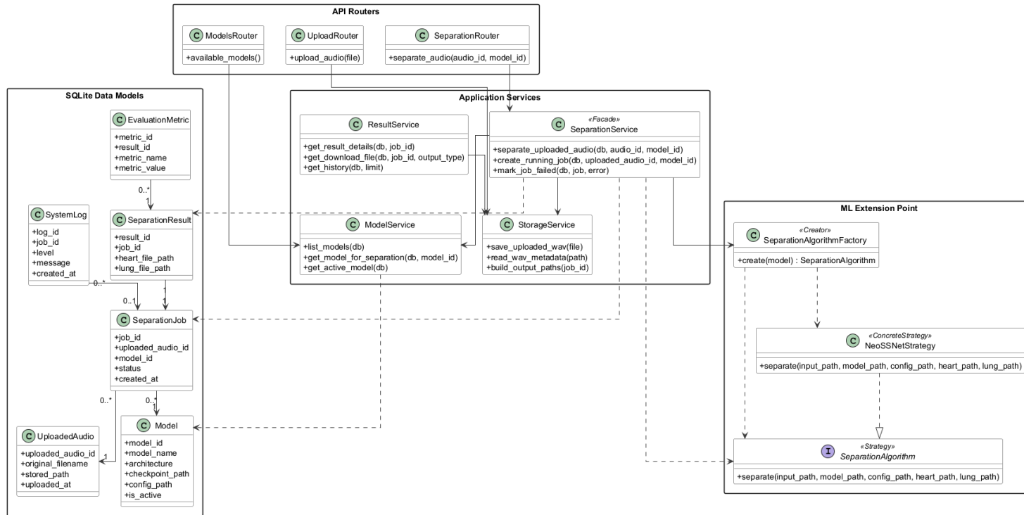
Figure 2.2: Overall System UML Class Diagram
