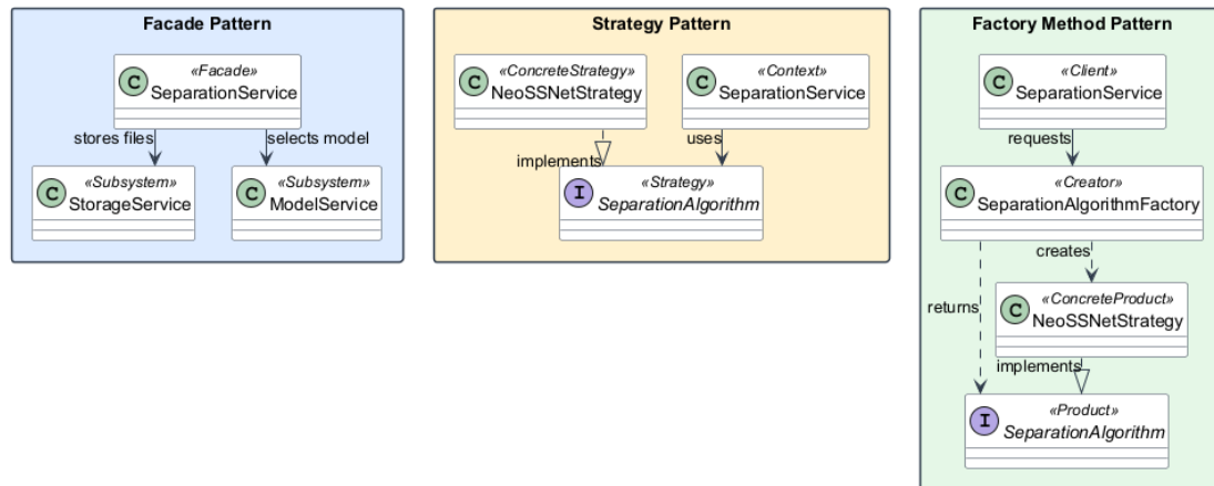
Figure 2.3: Design Pattern Location Overview
