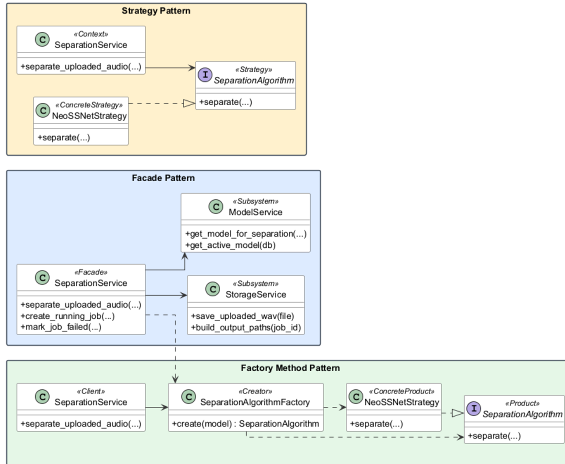
Figure 2.2: Pattern-Grouped Overall UML Class Diagram
