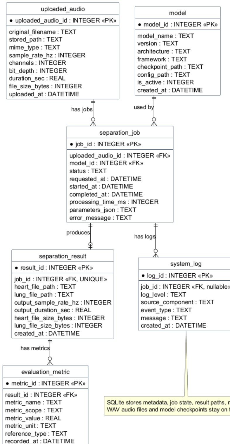
Figure 2.4: Entity Relationship Diagram
